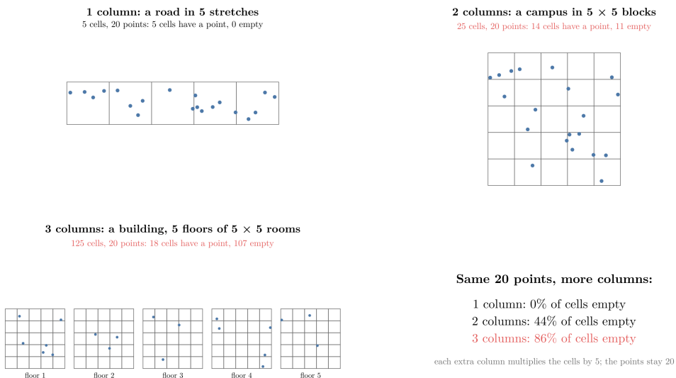
Figure 3: The same 20 points in 1, 2 and 3 features
