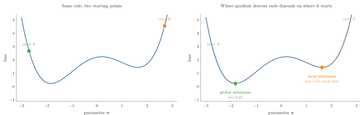
Figure 10: Two runs of gradient descent on the same non-convex curve (learning rate 0.07). Start A reaches the global minimum; start B stops in the local minimum. The ball-rolling picture follows 3Blue1Brown, “Gradient descent, how neural networks learn”.
