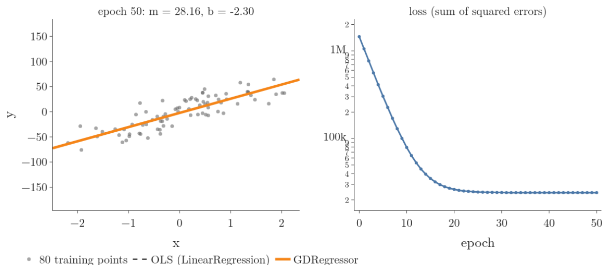
Figure 8: The GDRegressor class at work on the 80 training points: the line after each epoch (orange) closing in on the OLS line (dashed), and the loss per epoch on a log scale.
