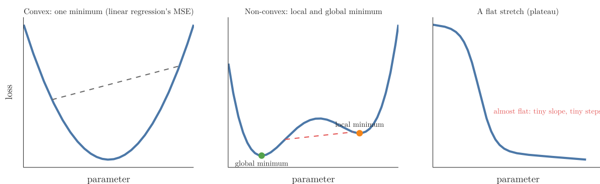
Figure 9: Convex and non-convex loss functions
