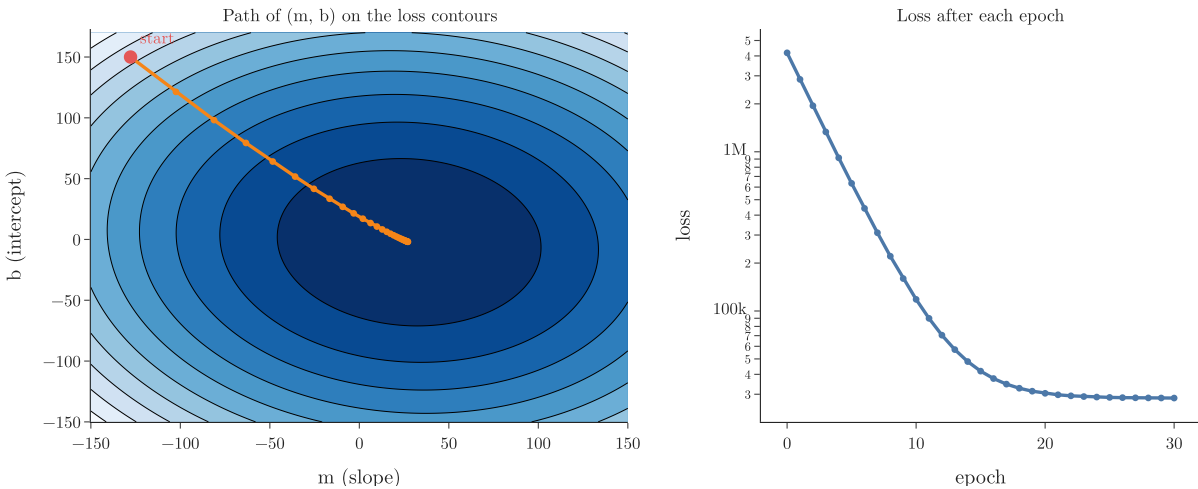
Figure 7: Gradient descent on m and b : the path and the loss per epoch
