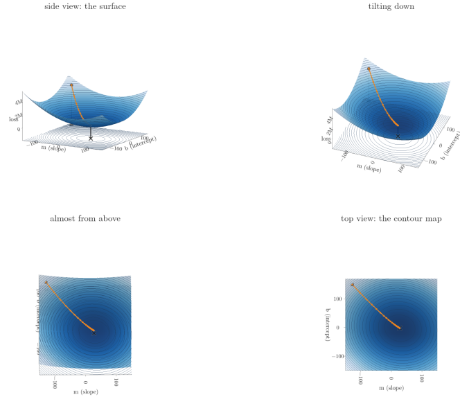
Figure 6: The loss surface L(m, b) of the 100 points, seen from the side and tilted to the top view, with the 30-epoch descent path in orange. The final frame is the contour map of Figure 7.
