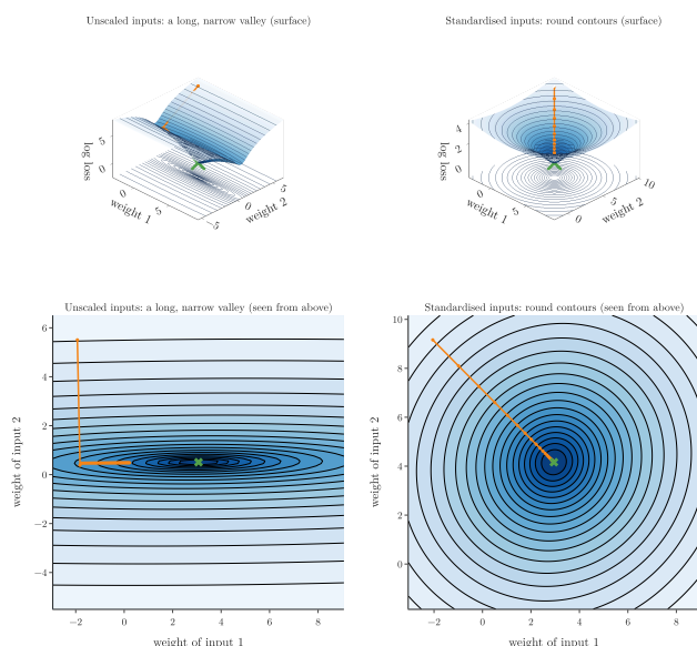
Figure 11: The effect of scaling the inputs on gradient descent
