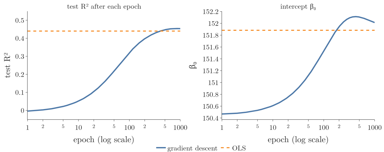
Figure 4: What the GDRRegressor code produces on the diabetes data, learning rate 0.5. Left: test R^2 after each epoch against the OLS value. Right: the intercept against the OLS intercept. Both axes of epochs use a log scale.
