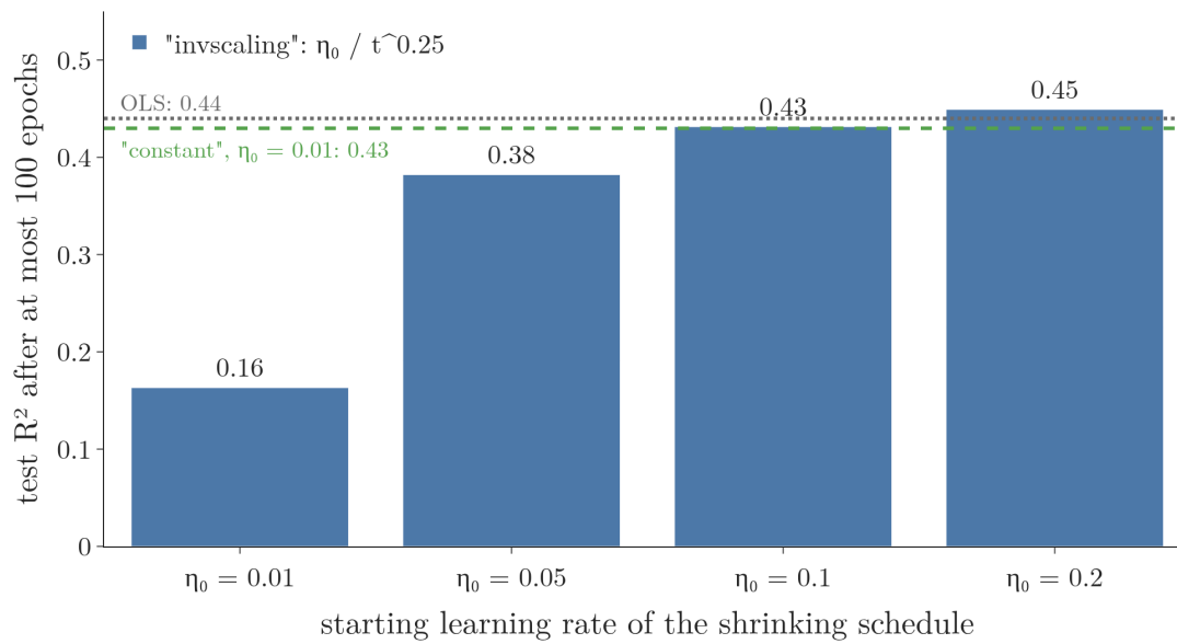
Figure 8: Test R^2 of SGDRegressor on the diabetes data after at most 100 epochs, with the shrinking “invscaling” schedule at four starting rates (bars), against the constant rate 0.01 (dashed green) and OLS (dotted grey).
