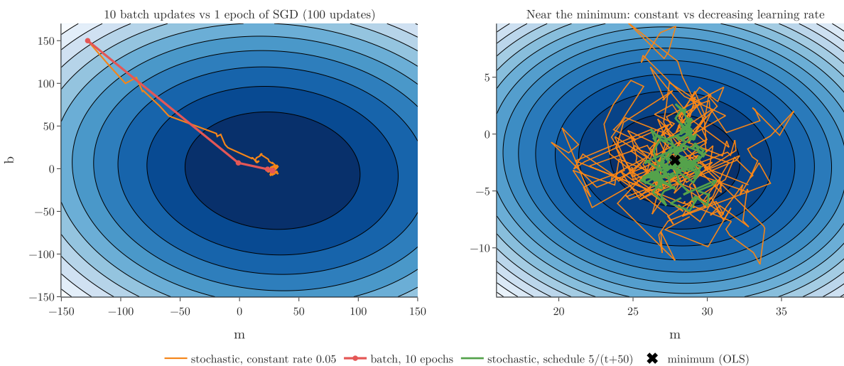
Figure 5: Batch vs stochastic paths, and the effect of a learning schedule
