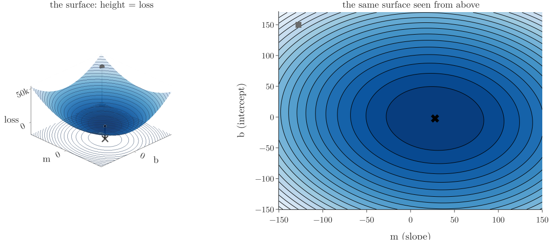
Figure 2: The loss surface of the 100-point example (left) and the same surface seen from above, a contour map (right). Grey square: the start m = -127.8 , b = 150 . Black cross: the best line.
