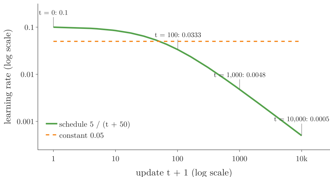
Figure 7: The learning schedule 5 / (t + 50) against a constant rate of 0.05, both axes on a log scale
