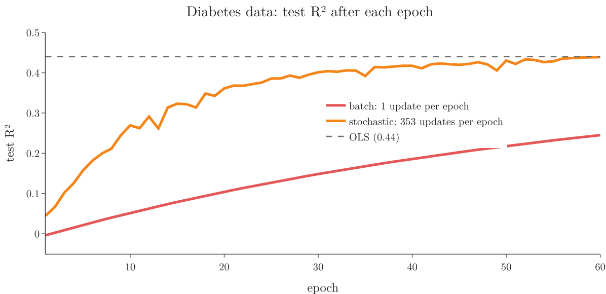
Figure 4: Test R^2 after each epoch: batch vs stochastic
