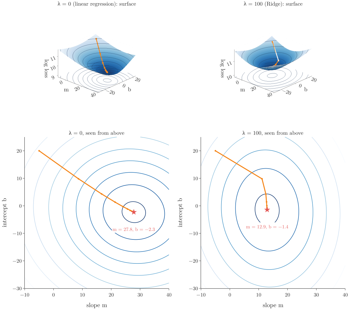
Figure 4: Gradient descent on the loss with \lambda = 0 and \lambda = 100
