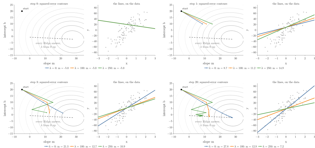
Figure 3: Gradient descent with \lambda = 0, 100 and 250 from the same start. Left: the paths on the squared-error contours; the dashed curve holds every Ridge answer as \lambda grows from 0. Right: each path's current line on the data
