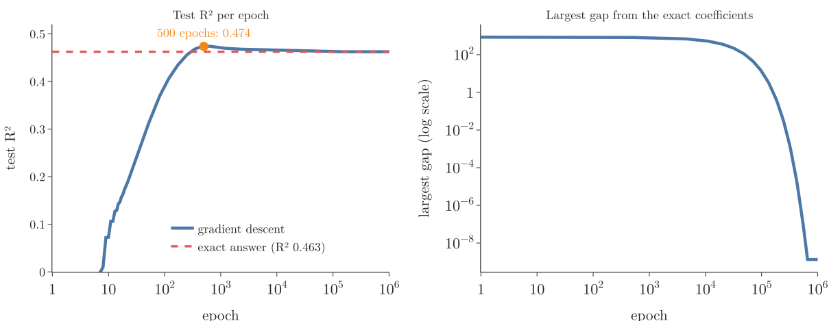
Figure 7: Test R^2 and distance from the exact answer, per epoch
