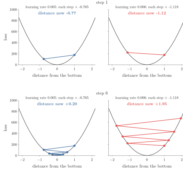
Figure 5: One direction of the loss bowl, curvature 353. Left: learning rate 0.005, each step multiplies the distance from the bottom by -0.765 , so the jumps shrink. Right: learning rate 0.006, each step multiplies it by -1.118 , so the jumps grow
