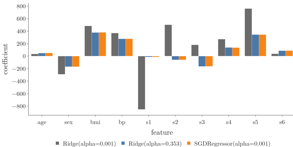
Figure 8: Coefficients on the diabetes training data (353 observations): Ridge with \alpha 0.001 (grey) and 0.353 (blue), and SGDRegressor with \alpha 0.001 run for 50,000 epochs (orange). The orange bars match the blue ones.
