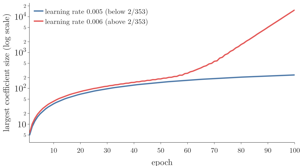
Figure 6: The largest coefficient of the from-scratch code per epoch on the diabetes data, alpha 0.001. Learning rate 0.005 (blue, below the limit 2/353 ) settles; 0.006 (red, above it) grows to about 15,000 after 100 epochs. Log scale.
