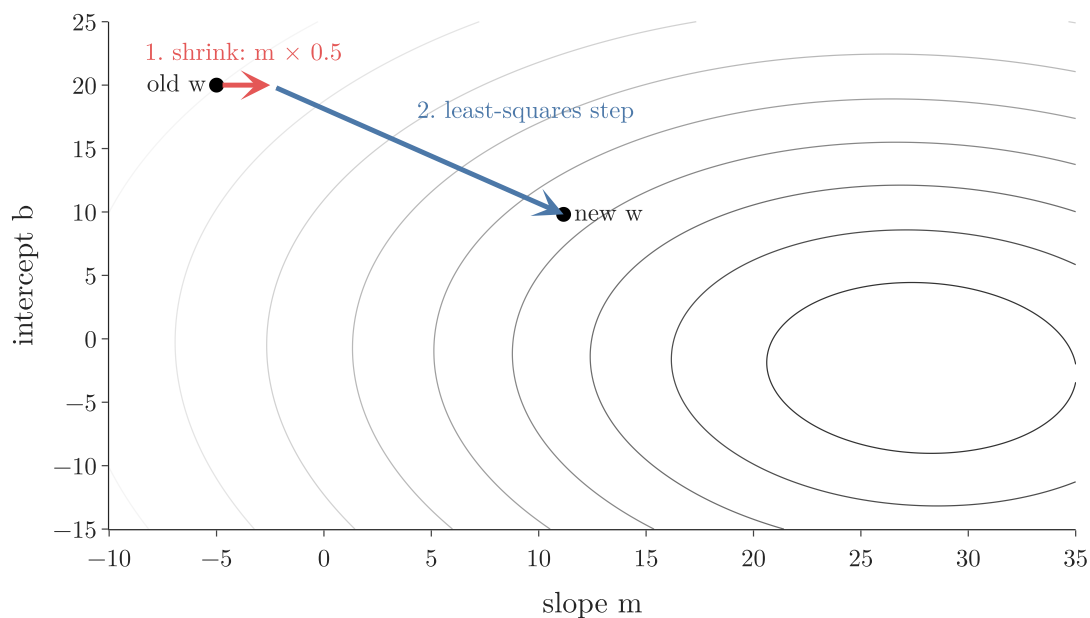
Figure 2: One Ridge step in two parts, on the squared-error contours: shrink the slope by 1 - \eta\lambda = 0.5 (red), then take the ordinary least-squares step (blue). The intercept is not shrunk
