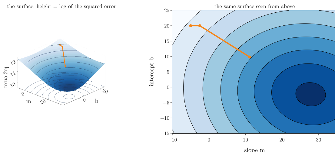
Figure 1: The squared-error surface of the one-feature example (left) and the same surface seen from above, a contour map (right). Orange: the Ridge step of Figure 2, from the start (-5, 20) through the shrink to the new point (11.2, 9.8) .
