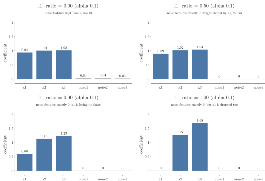
Figure 7: The six Elastic Net coefficients on the data of Figure 6 while l1_ratio grows from 0 to 1 at alpha 0.1. The noise coefficients are small but not 0 at the Ridge end and exactly 0 from l1_ratio 0.5 on. The three copies share the weight until the Lasso end, where x_1 loses its share and is dropped
