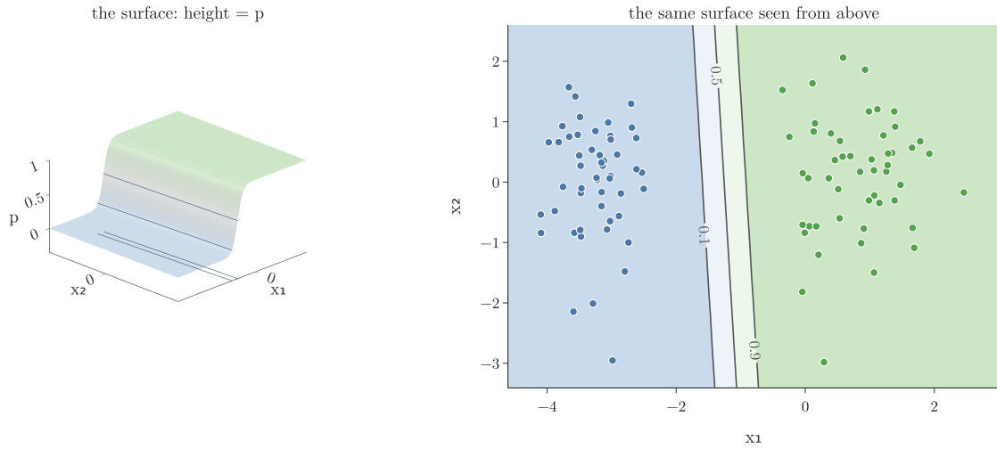
Figure 7: The probability surface of the model after 50,000 epochs on the perfectly separated points (left) and the same surface seen from above, a contour map with the lines p = 0.1, 0.5, 0.9 and the data (right).
