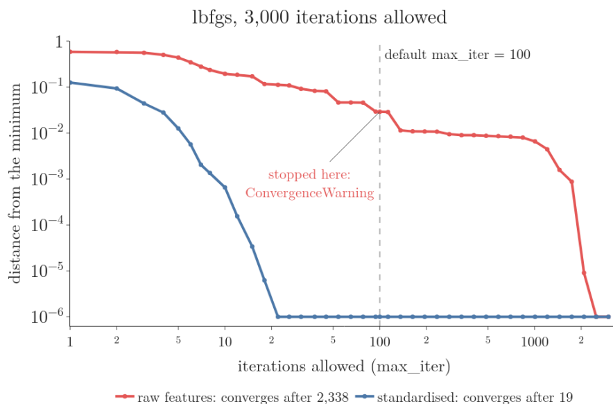
Figure 6: lbfgs on raw (red) and standardised (blue) breast-cancer features: distance from the minimum against iterations allowed. Points at the bottom are within one millionth of the minimum. The dashed line is the default max_iter = 100
