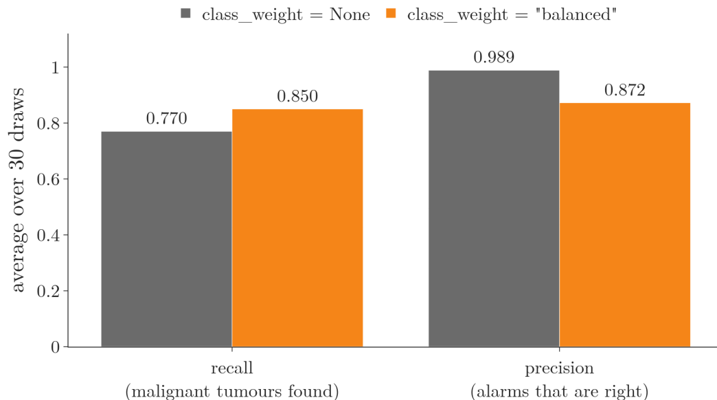
Figure 7: Recall and precision on the malignant class, averaged over 30 draws: “balanced” finds more malignant tumours (recall 0.770 to 0.850) but raises more false alarms (precision 0.989 to 0.872)
