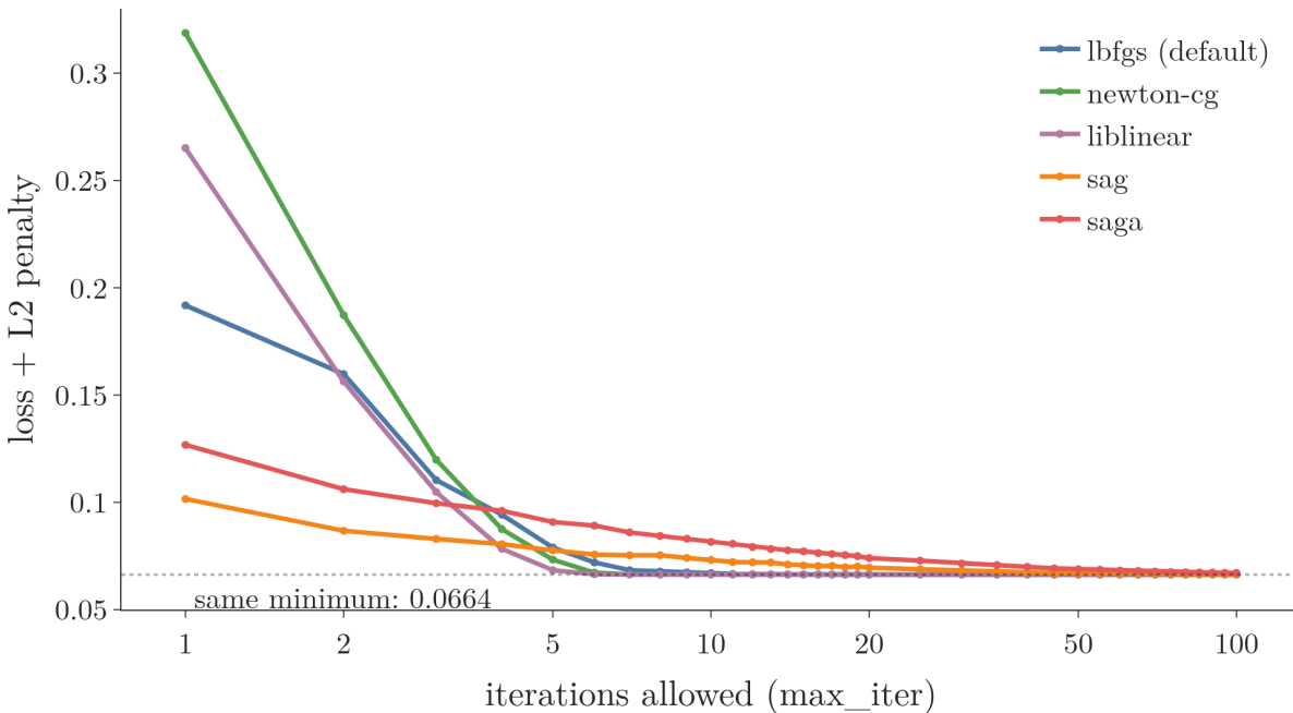
Figure 5: Five solvers on the standardised breast-cancer data (L2, C = 1 ): log loss plus penalty after k iterations. All reach the same minimum, 0.0664
