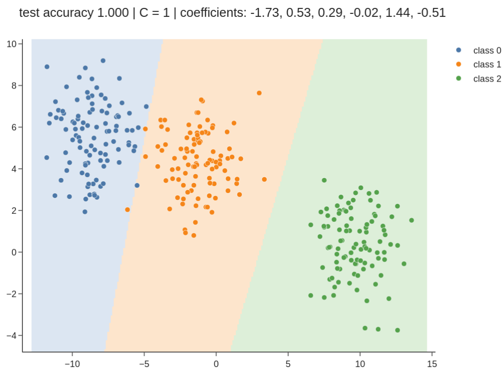
Figure 8: The playground on the three-class dataset with the default settings
