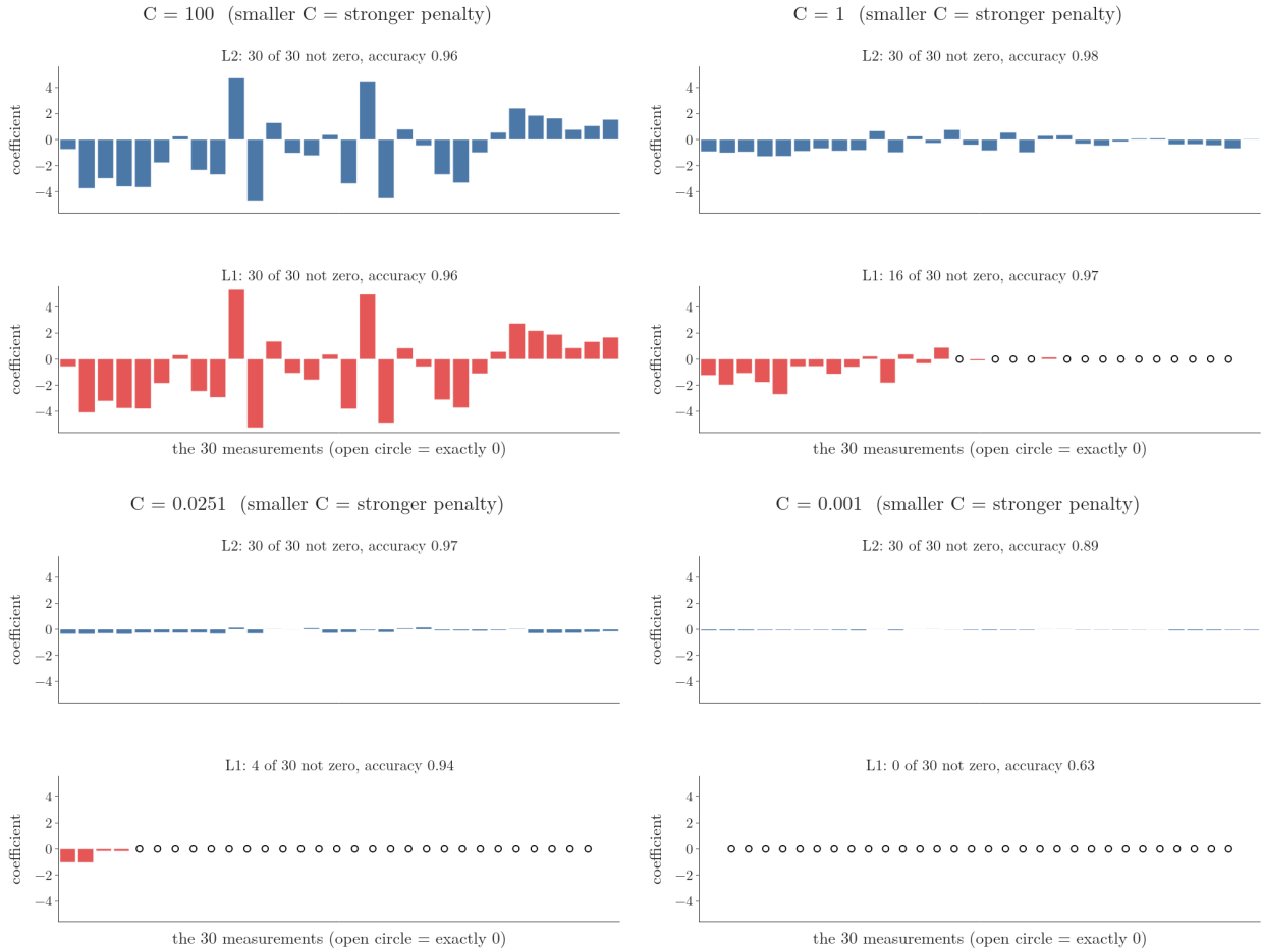
Figure 4: The 30 coefficients on the breast-cancer data as C falls from 100 to 0.001, for L2 (top) and L1 (bottom); titles give the 5-fold CV accuracy
