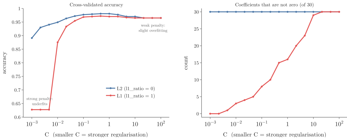
Figure 3: Cross-validated accuracy and number of non-zero coefficients against C
