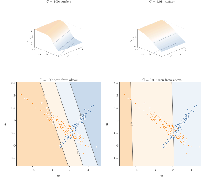
Figure 1: The probability surface of the 300 points for C = 100 (left) and C = 0.01 (right), each with the same surface seen from above, a contour map with the lines p = 0.1, 0.5, 0.9 .
