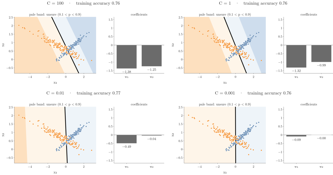
Figure 2: C falls from 100 to 0.001 on a two-feature dataset. Left: the decision boundary (black) and the pale band where the predicted probability is between 0.1 and 0.9. Right: the two coefficients. As C falls, the coefficients shrink towards 0, the unsure band widens until it covers nearly all the points, and the boundary turns
