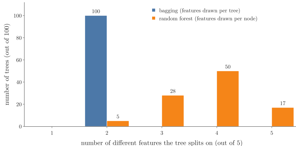
Figure 4: How many different features each of 100 trees splits on, out of 5, with max_features=2
