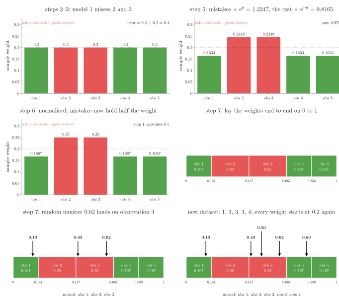
Figure 4: The 5 sample weights through one stage of the worked example: equal at 0.2, observations 2 and 3 misclassified (error 0.4, \alpha 0.2027), multiplied by e^\alpha or e^{-\alpha} , normalised, then laid end to end on the line from 0 to 1, where five random numbers pick the new dataset
