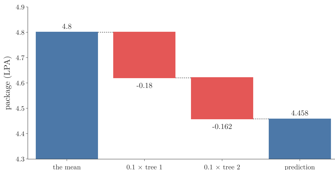
Figure 6: The prediction for the new student (IQ 60, CGPA 4.9): the mean 4.8, then 0.1 times each tree's output, -0.18 and -0.162 , giving 4.458. The axis starts at 4.3 so the small steps show
