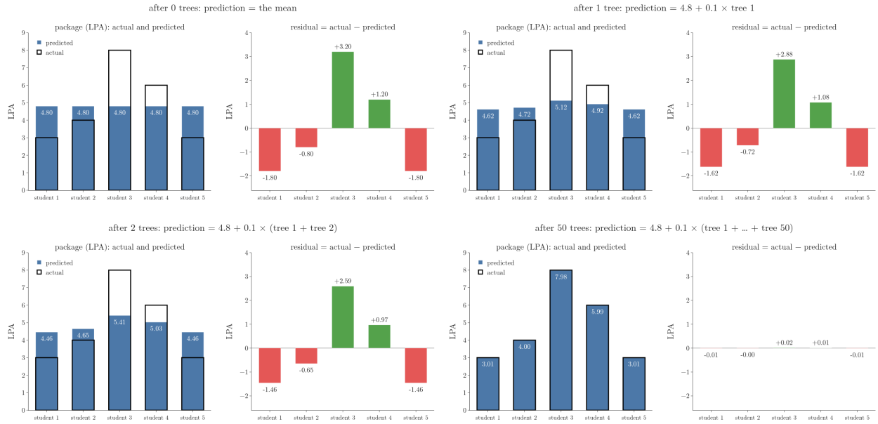
Figure 5: Gradient boosting on the five students, learning rate 0.1. Left: actual package (outline) and the model's prediction (blue bar). Right: the residuals the next tree is trained on
