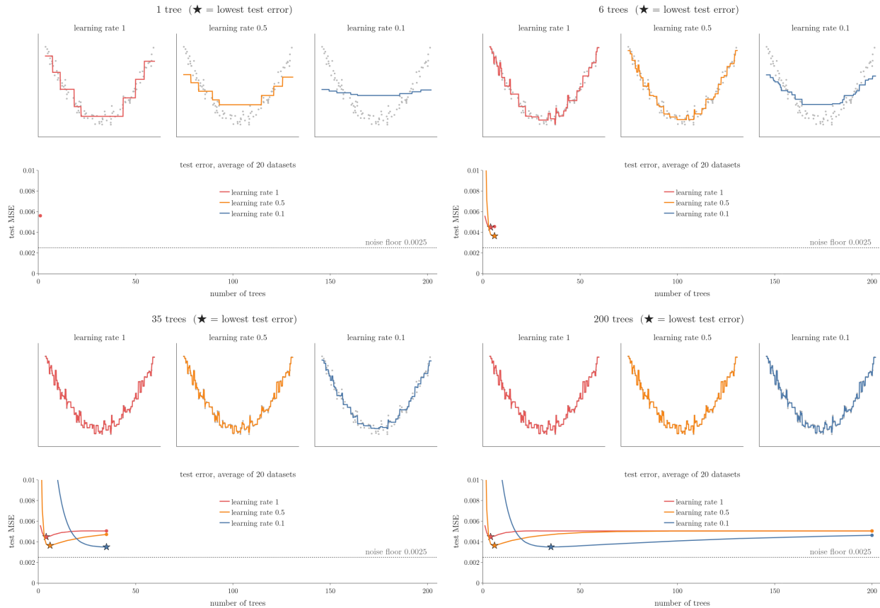
Figure 9: Gradient boosting with learning rates 1, 0.5 and 0.1 (8 leaves per tree), tree by tree. Top: the model on the curve data. Bottom: test error averaged over 20 fresh datasets; stars mark each learning rate’s lowest test error; the dotted line is the noise floor
