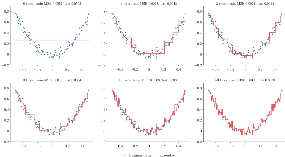
Figure 8: The model after 0, 1, 2, 3, 10 and 50 trees (learning rate 1, 8 leaves per tree), with training and test error
