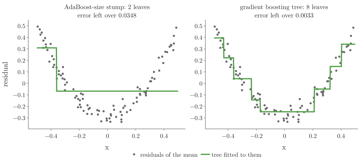
Figure 10: The residuals of the mean on the curve data, fitted by a stump with 2 leaves (left) and by a tree with 8 leaves (right); titles give the squared error left over
