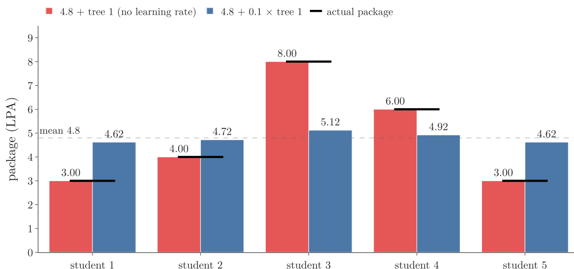
Figure 4: Five students after the mean plus tree 1: added in full (red), every prediction equals the actual package; added with learning rate 0.1 (blue), every prediction moves one tenth of the way from 4.8
