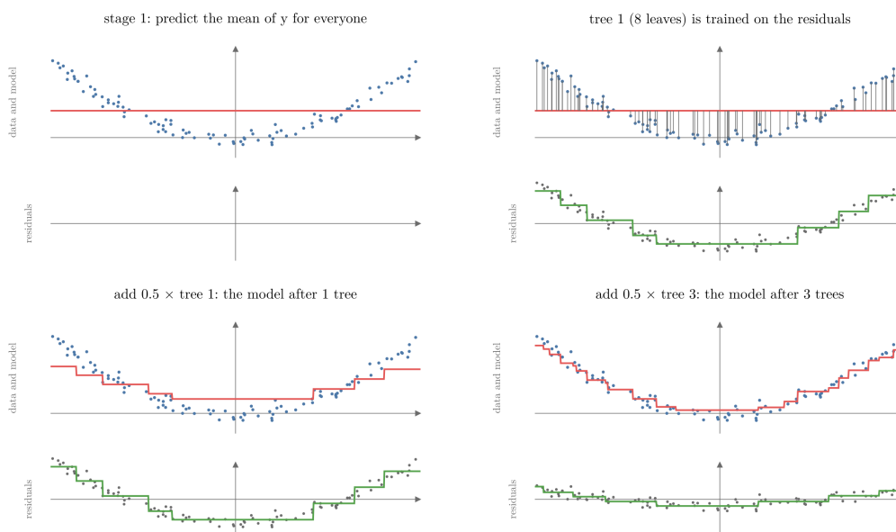
Figure 7: Gradient boosting on the curve, learning rate 0.5: residuals of the current model (grey), the tree trained on them (green), and the model after adding half of it (red)
