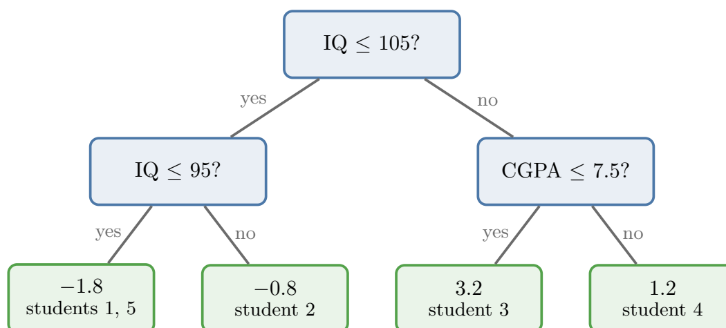
Figure 3: Tree 1, trained on the residuals: each leaf holds the residual of the students that reach it
