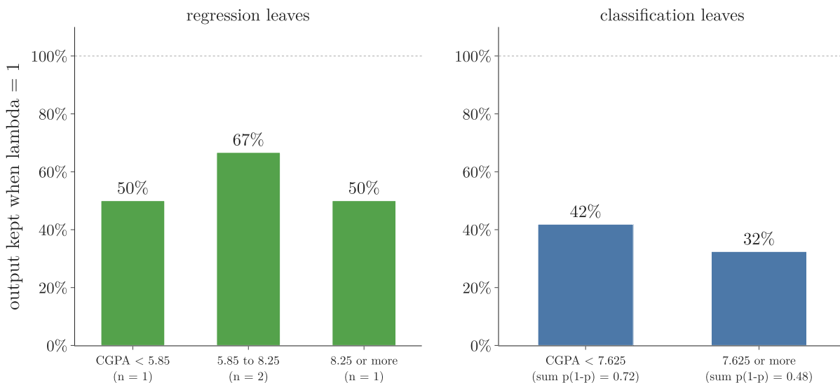
Figure 7: The share of each leaf output that survives \lambda = 1 . Regression leaves keep n/(n + 1) : 50 or 67 percent. Classification leaves keep \sum p(1 - p) / (\sum p(1 - p) + 1) : only 42 and 32 percent
