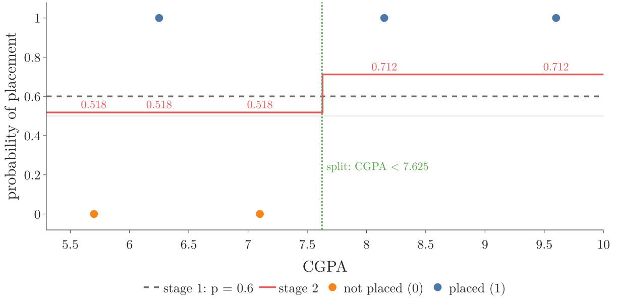
Figure 5: Stage 1 gives every student probability 0.6; after one tree the probability drops to 0.518 below CGPA 7.625 and rises to 0.712 above it
