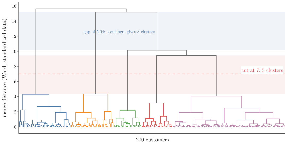
Figure 8: Ward dendrogram of the 200 customers (standardized features); the cut at 7 gives 5 clusters
