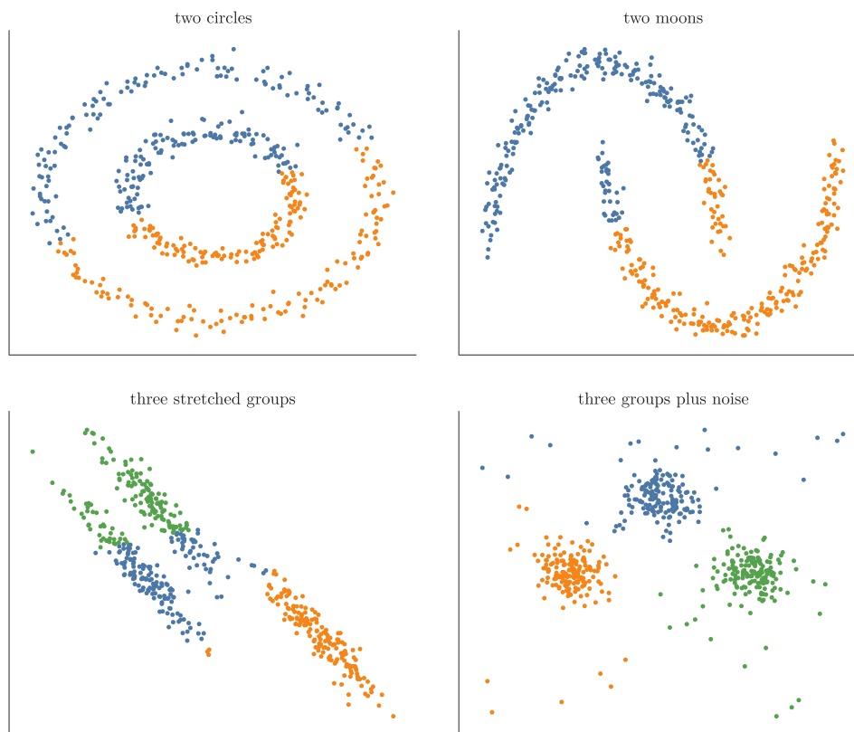
Figure 2: k-means ( k = 2 or 3 ) on four datasets: one colour per cluster found
