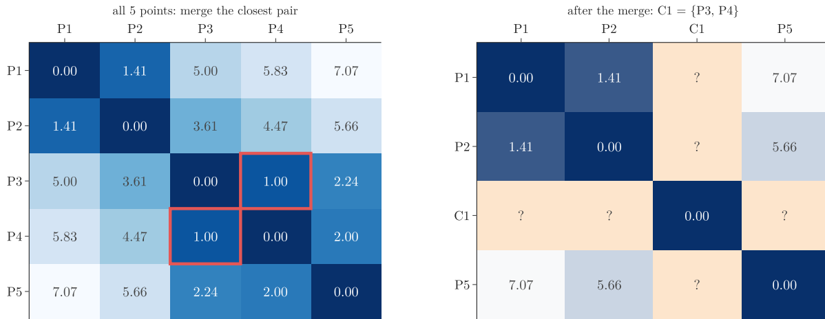
Figure 4: The proximity matrix of the five points. Left: all distances, with the smallest off the diagonal (P3 to P4, 1.00) outlined. Right: after merging P3 and P4 into C_1 , the distances between unchanged points stay; the row and column of C_1 wait for a linkage rule
