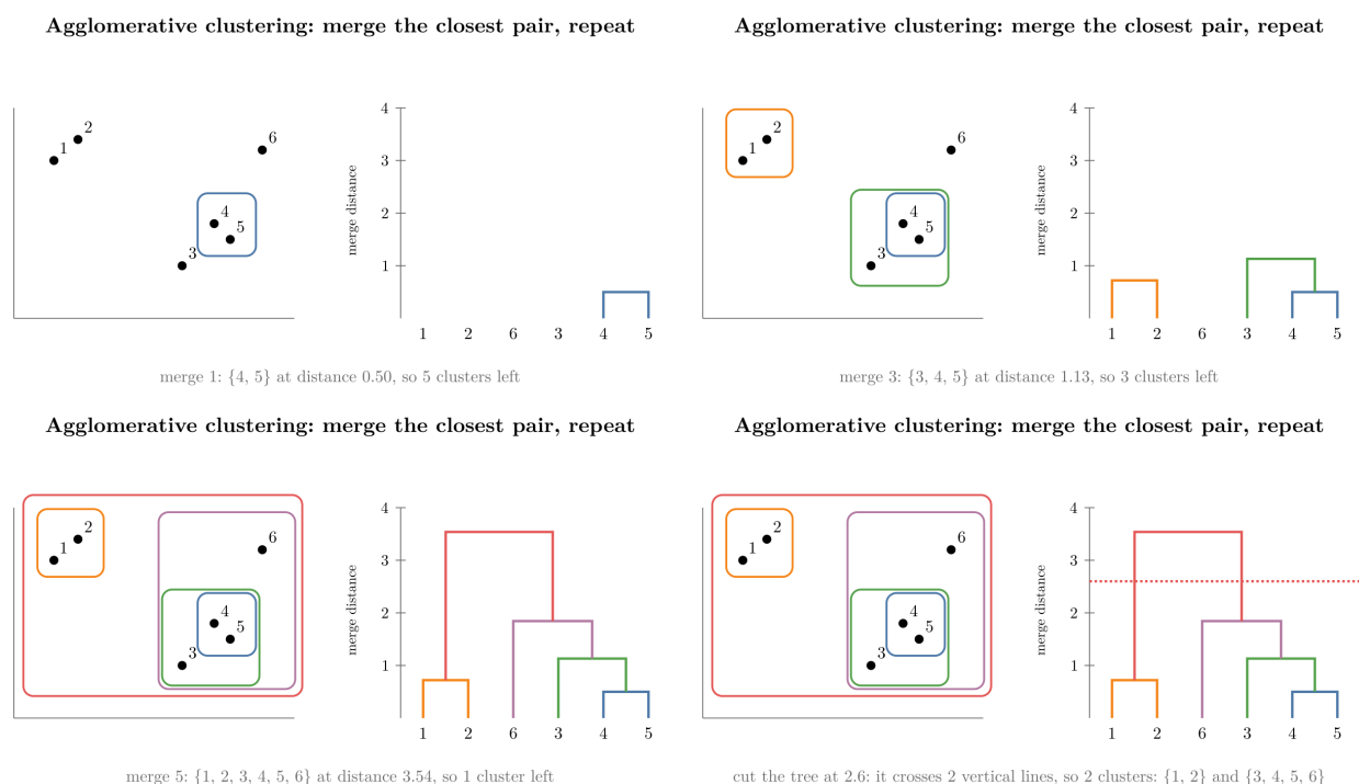
Figure 1: Agglomerative clustering on 6 points: each merge (left) adds one link to the dendrogram (right); a cut through the tree gives the clusters
