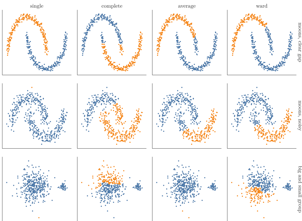
Figure 7: Single, complete, average and Ward linkage (2 clusters) on moons with a clear gap, noisy moons, and a big and a small group
