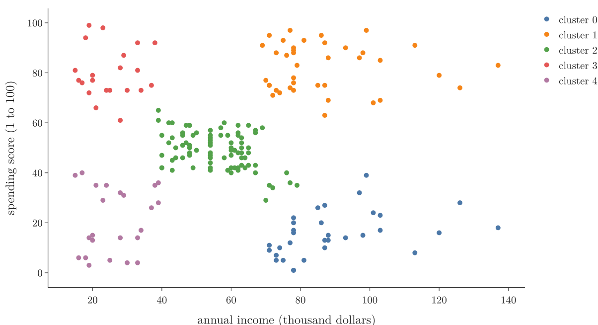
Figure 9: The 200 customers in the 5 clusters found by Ward linkage
