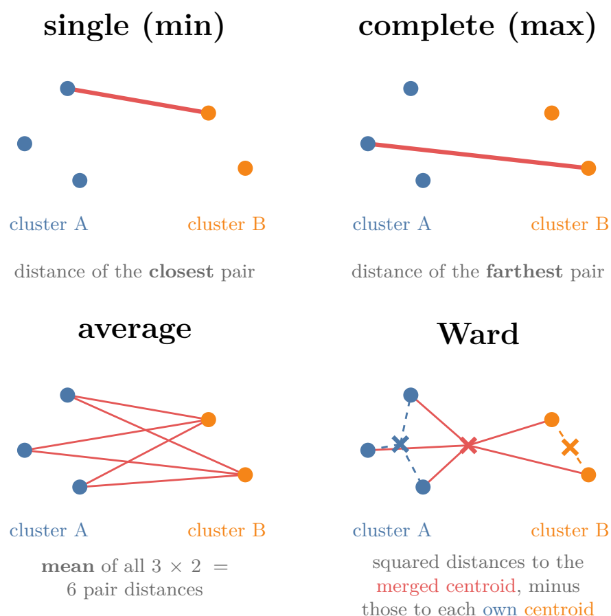
Figure 5: The four linkages: how the distance between cluster A and cluster B is measured
