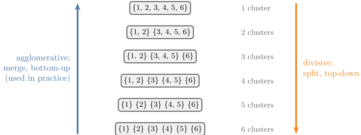
Figure 3: The two directions on the six points of section 5. Agglomerative clustering reads the list bottom-up, merging the two closest clusters at each step; divisive clustering reads it top-down, splitting one cluster at each step
