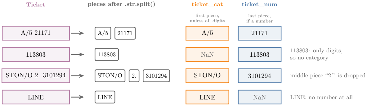
Figure 3: Each ticket split at its spaces: the first piece becomes the category, the last piece the number
