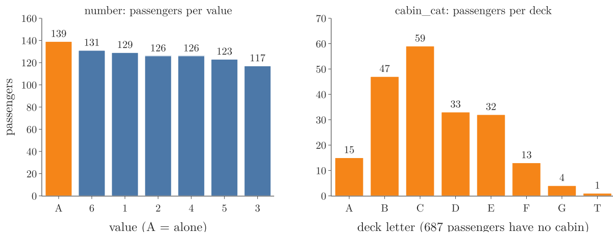
Figure 2: Left: passengers per value of the mixed column number . Right: passengers per deck after splitting Cabin
