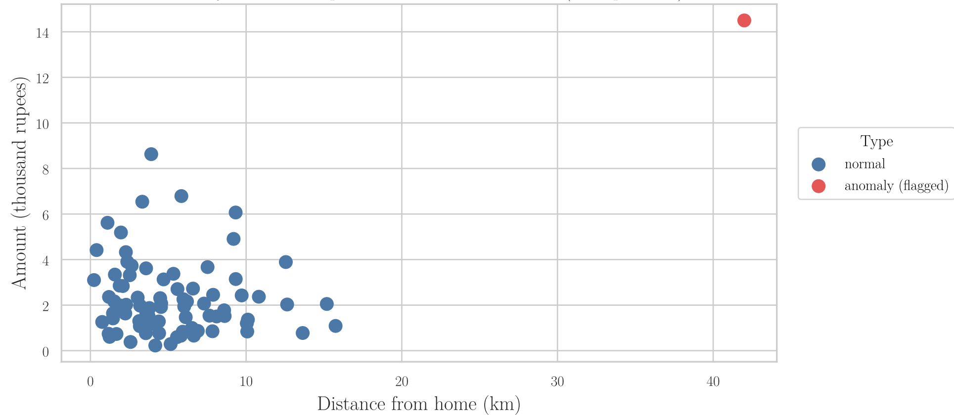
Anomaly detection: a point far from all the others (example data)
