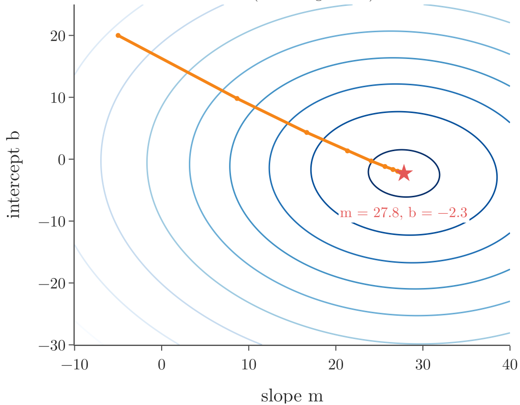
\lambda = 0 (linear regression)
