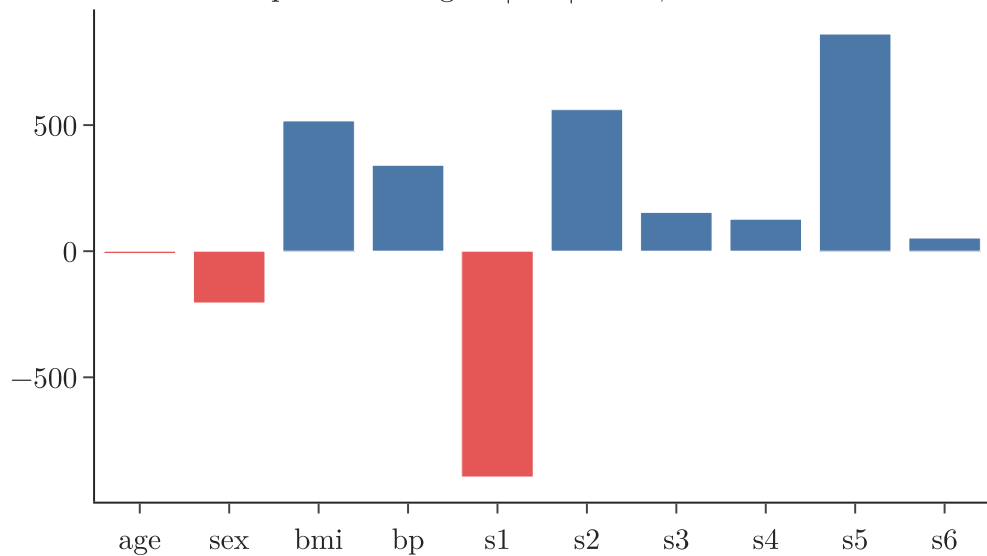
alpha = 0: largest |coef| 895.6, test R 2 0.44
