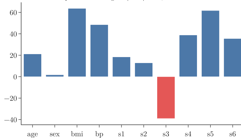
alpha = 10: largest |coef| 63.7, test R 2 0.15
