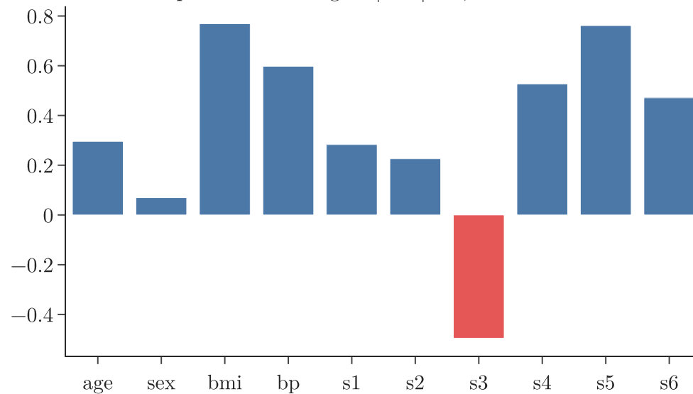
alpha = 1000: largest |coef| 0.8, test R 2 -0.01
