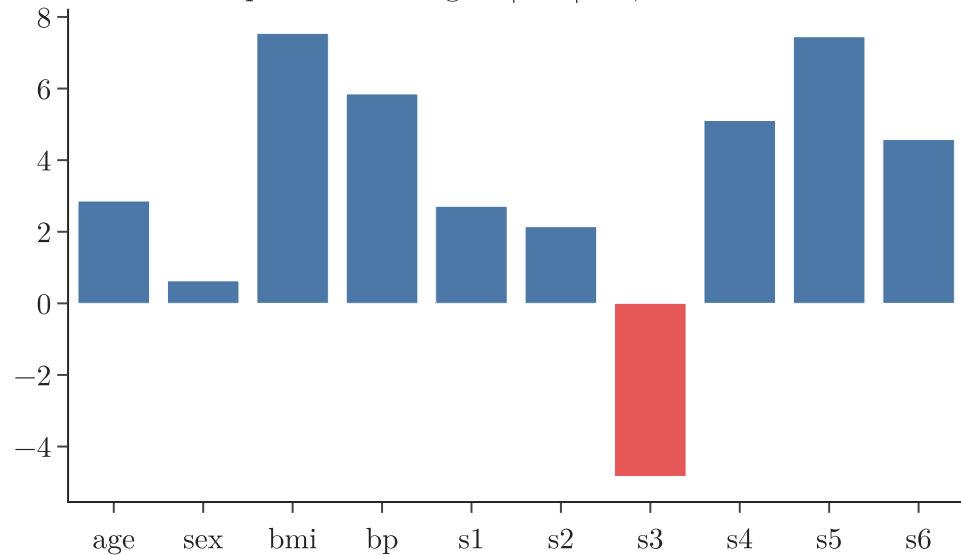
alpha = 100: largest |coef| 7.5, test R 2 0.01
