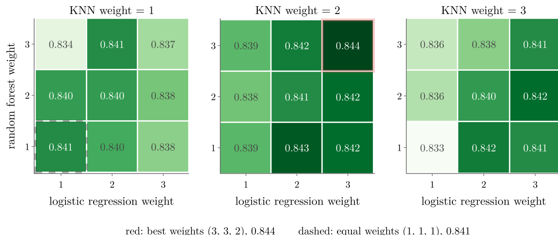
Figure 6: Soft-vote accuracy on the heart disease data for all 27 weight triples (each weight 1 to 3). Red outline: the best, (3, 3, 2), 0.844. Dashed outline: equal weights, 0.841. Every cell lies between 0.833 and 0.844
