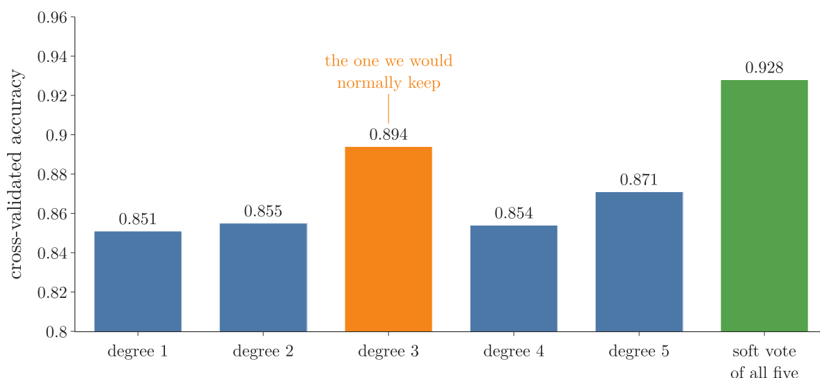
Figure 7: Polynomial-kernel SVMs of degree 1 to 5, each alone, and all five in one soft vote (10-fold cross-validation)
