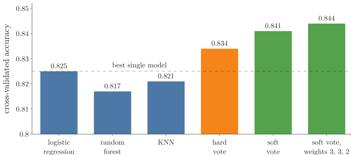
Figure 5: Cross-validated accuracy on the heart disease data: the three base models, the hard and soft vote, and the soft vote with the best weights. The dashed line is the best single model
