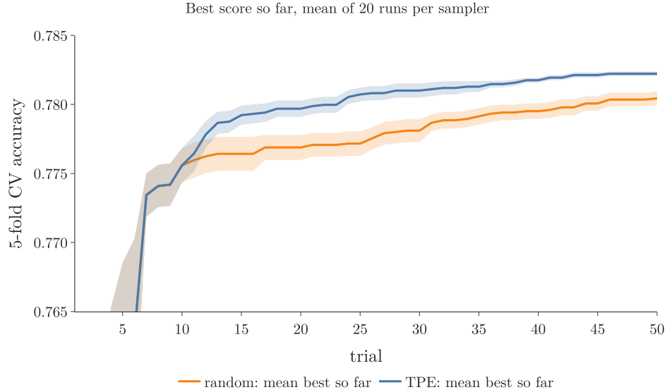
Figure 6: Best 5-fold CV accuracy so far, averaged over 20 runs of each sampler on the SVM search; the bands are \pm one standard error
