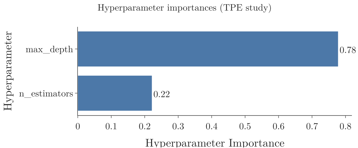
Figure 10: Hyperparameter importances of the TPE study
