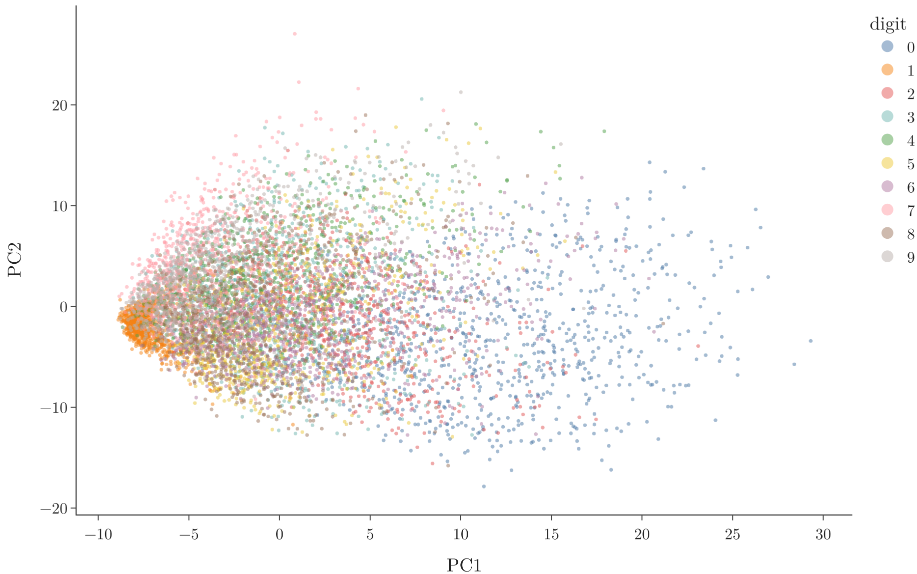
MNIST test images on the first two principal components
