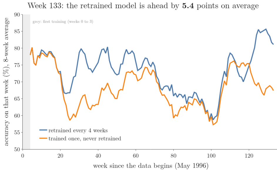
Figure 4: A batch model on the Electricity market data. Orange: trained once on the first 4 weeks and never retrained. Blue: retrained from scratch on all data so far, every 4 weeks. Each line is the accuracy on each following week, averaged over 8 weeks.
