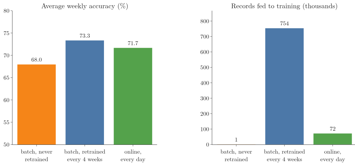
Figure 9: Accuracy against training work on the Electricity market data, weeks 4 to 133. Training work counts each record once each time it is fed to training.
