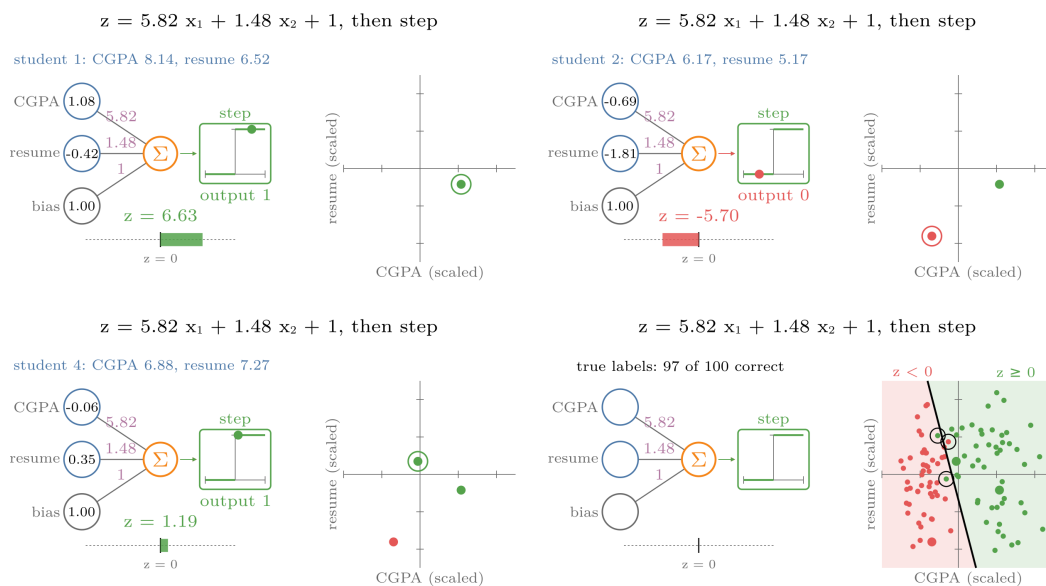
Figure 3: Prediction with a trained perceptron, z = 5.82x_1 + 1.48x_2 + 1 on standardized CGPA and resume score. For each student the inputs flow in, z fills a bar (green if positive, red if negative), the step function fires 1 or 0, and the student lands on the plane in that colour. At the end all 100 students appear with the line z = 0 between the two regions
