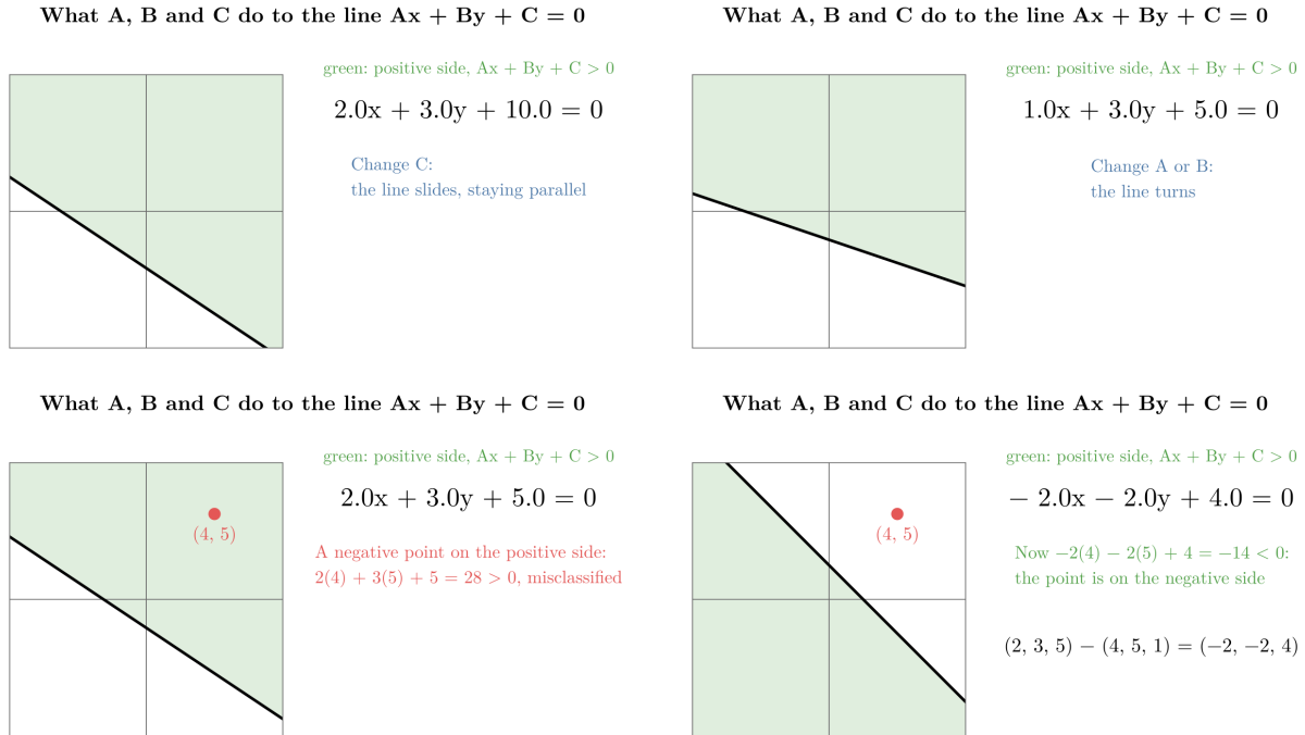
Figure 2: The line 2x + 3y + 5 = 0 . First C changes, then A , then B . Then the negative point (4, 5) , which sits on the positive (green) side, is subtracted from the coefficients
