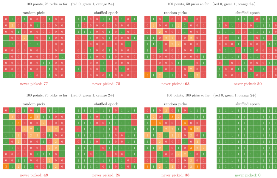
Figure 5: Each cell is one of 100 training points, and its number counts how often it has been picked. Left: 100 random picks, as in the perceptron trick; 38 points are never picked while others are picked 2 or 3 times. Right: one shuffled epoch; every point is picked exactly once
