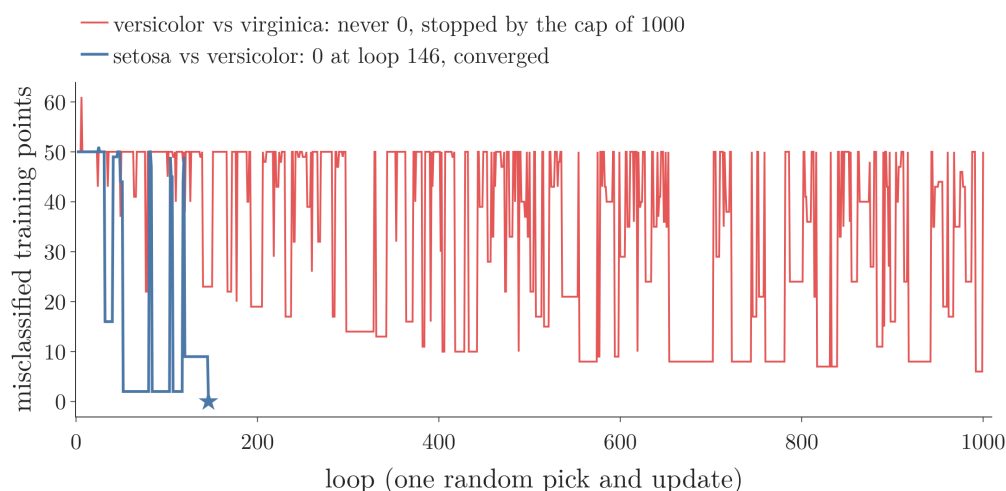
Figure 4: The perceptron trick on two pairs of Iris species (petal length and width, 100 flowers each, learning rate 0.1), counting the misclassified training points after every loop
