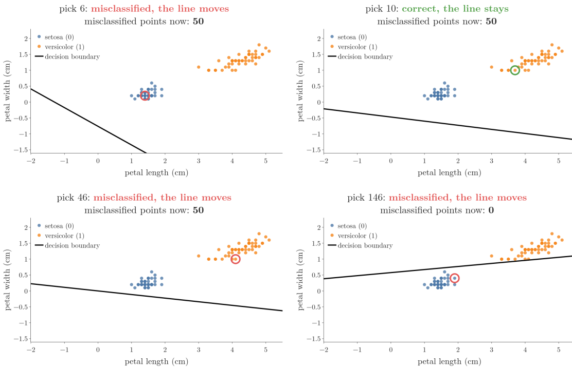
Figure 3: The perceptron trick pick by pick on Iris setosa and versicolor. The ring marks the picked flower: green when it is correctly classified, red when it is misclassified
