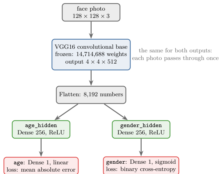
Figure 7: The age and gender model: one frozen VGG16 base, Flatten, and two branches with their own output and loss
