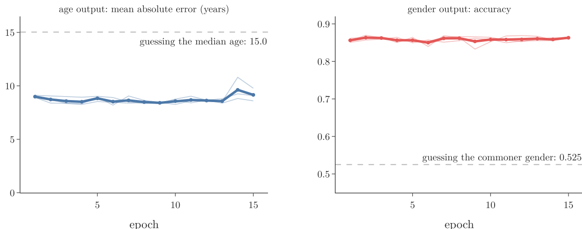
Figure 9: The two-output model on the test photos, epoch by epoch: the age error (left) and the gender accuracy (right). Thin lines: 3 seeds; thick lines: their mean; dashed: guessing
