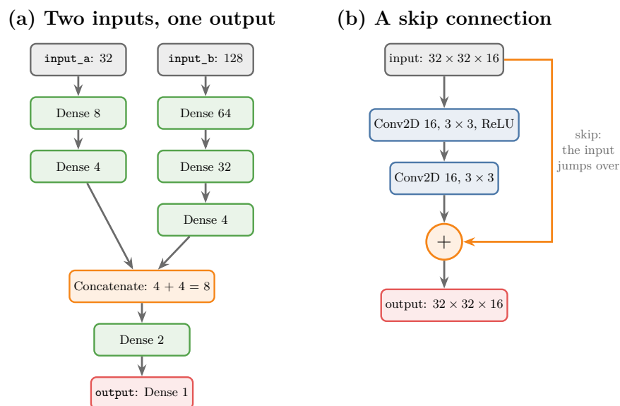
Figure 5: (a) Two inputs processed separately and joined by Concatenate . (b) A skip connection: the input jumps over two convolution layers and is added to their output
