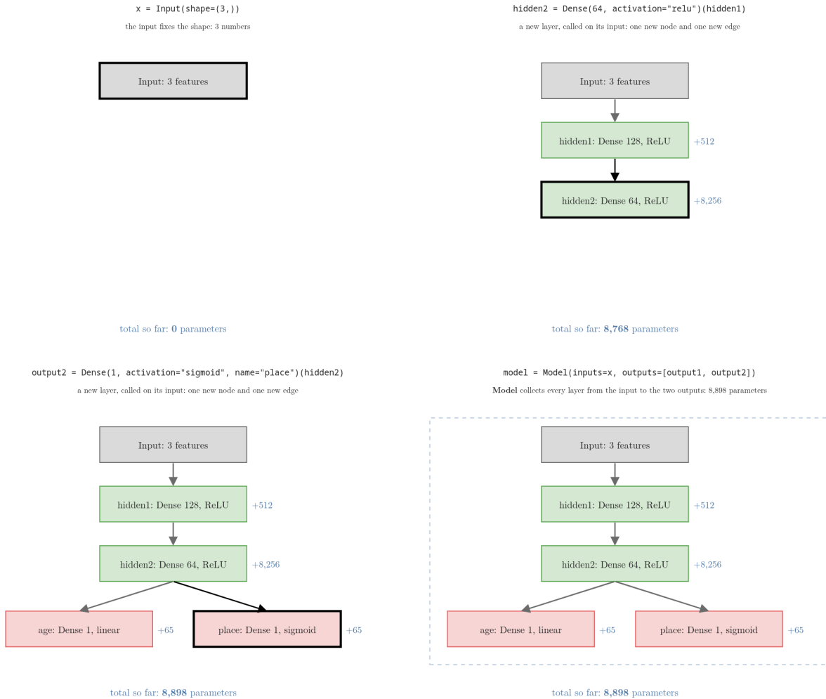
Figure 4: Building the model of Figure 3, one line of code per frame. Each call adds a node (black border) and the edge from its input; the blue number is the layer’s parameter count, and the running total reaches 8,898
