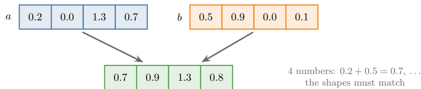
Figure 6: The same two vectors joined two ways. (a) Concatenate places them one after the other: 8 numbers. (b) Add sums them position by position: 4 numbers, so the two shapes must match
