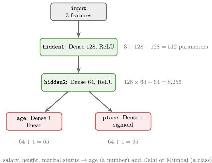
Figure 3: A functional model with one input and two outputs. Both outputs read the second hidden layer. The numbers are each layer’s parameters
