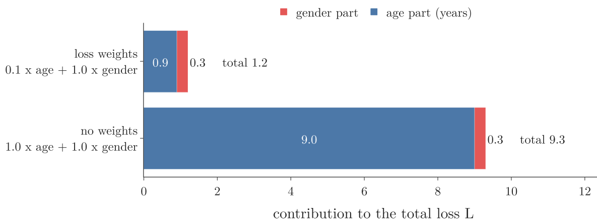
Figure 8: The worked example as bars. Without weights, the age part (9.0) is 30 times the gender part (0.3), so training would mostly reduce the age error. With a weight of 0.1 on age, the two parts are 0.9 and 0.3
