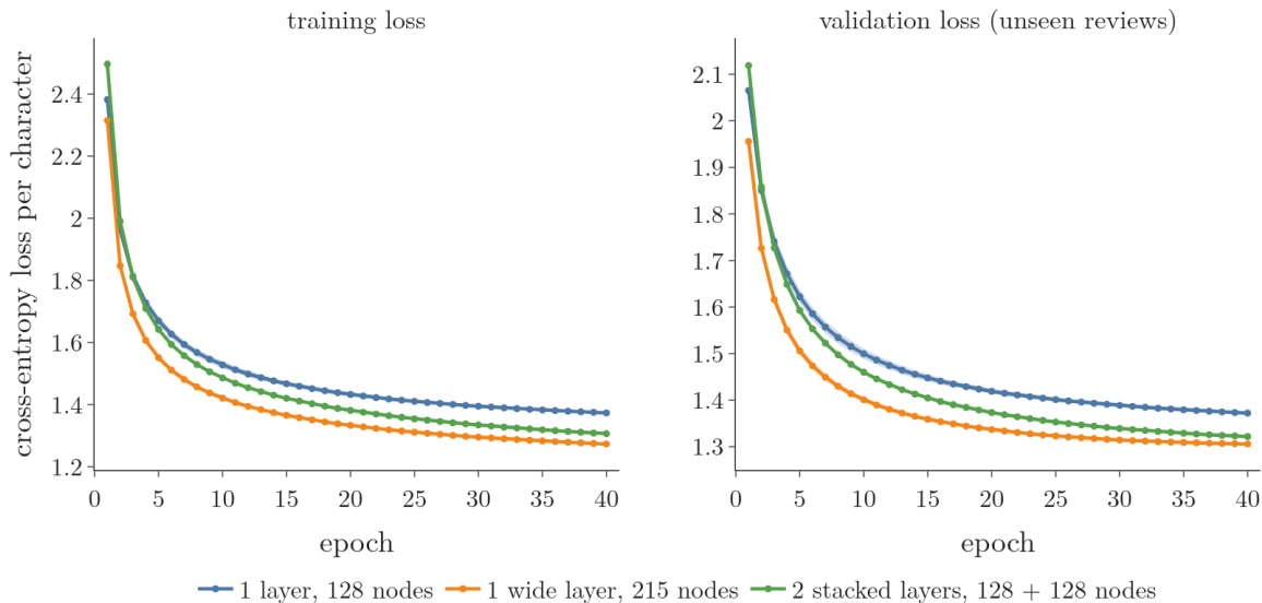
Figure 7: Training loss (left) and validation loss (right) per epoch, mean of 2 seeds (band: lower to higher seed). The loss is the cross-entropy per character, lower is better
