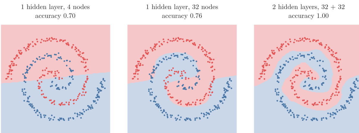
Figure 2: Three MLPs trained on the same two-arm spiral (400 points). The shading is the class each network predicts at each point of the plane; the edge between the two shades is the decision boundary. Accuracy on the training points, mean of 5 seeds; each map shows a typical seed
