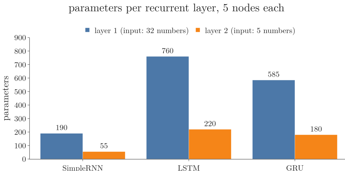
Figure 8: Parameters of each recurrent layer in the two-layer model of section 6 (5 nodes per layer), built from SimpleRNN, LSTM or GRU layers. Counts from Keras' model.summary() in the Notebook
