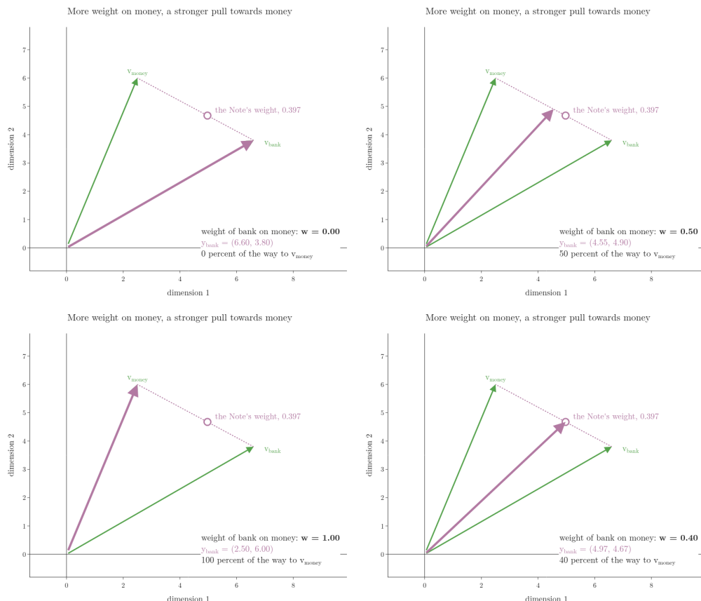
Figure 7: The weight w that “bank” puts on “money” slides from 0 to 1. The output y_{\text{bank}} (purple) slides along the dotted line from v_{\text{bank}} to v_{\text{money}} ; the open circle marks the weight our numbers give, 0.397
