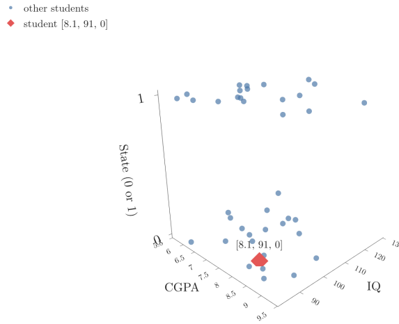
Figure 5: Each student is a point in 3D space
