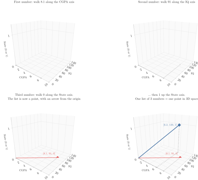
Figure 4: A list of three numbers read as a walk along three axes
