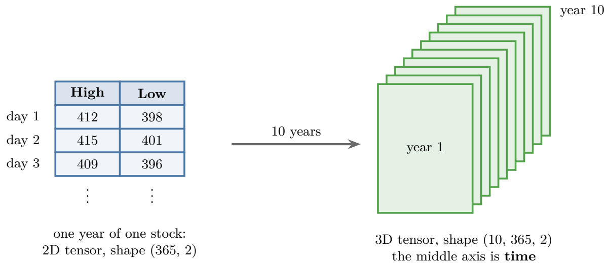
Figure 8: Stock prices as a 3D tensor
