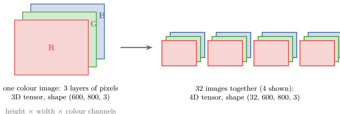
Figure 9: Images as tensors
