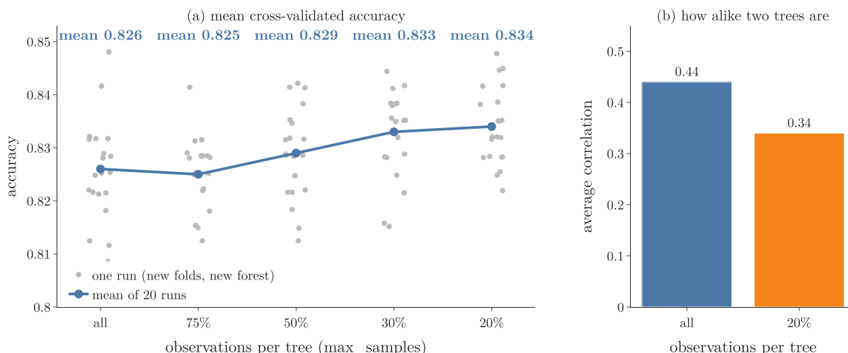
Figure 5: (a) Mean 10-fold cross-validated accuracy against the observations per tree ( max_samples ), 500 trees; each grey dot is one of 20 runs with new folds and a new forest. (b) Average correlation between two trees' predicted probabilities on the 61 test patients
