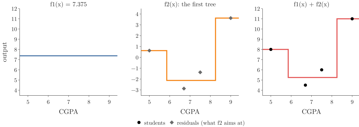
Figure 2: A boosting model as a sum of functions, on the four students of the XGBoost regression Note. Left: the base model f1 , the mean 7.375. Middle: the first tree f2 , fitted to the residuals (grey). Right: their sum, a staircase that passes through two of the students
