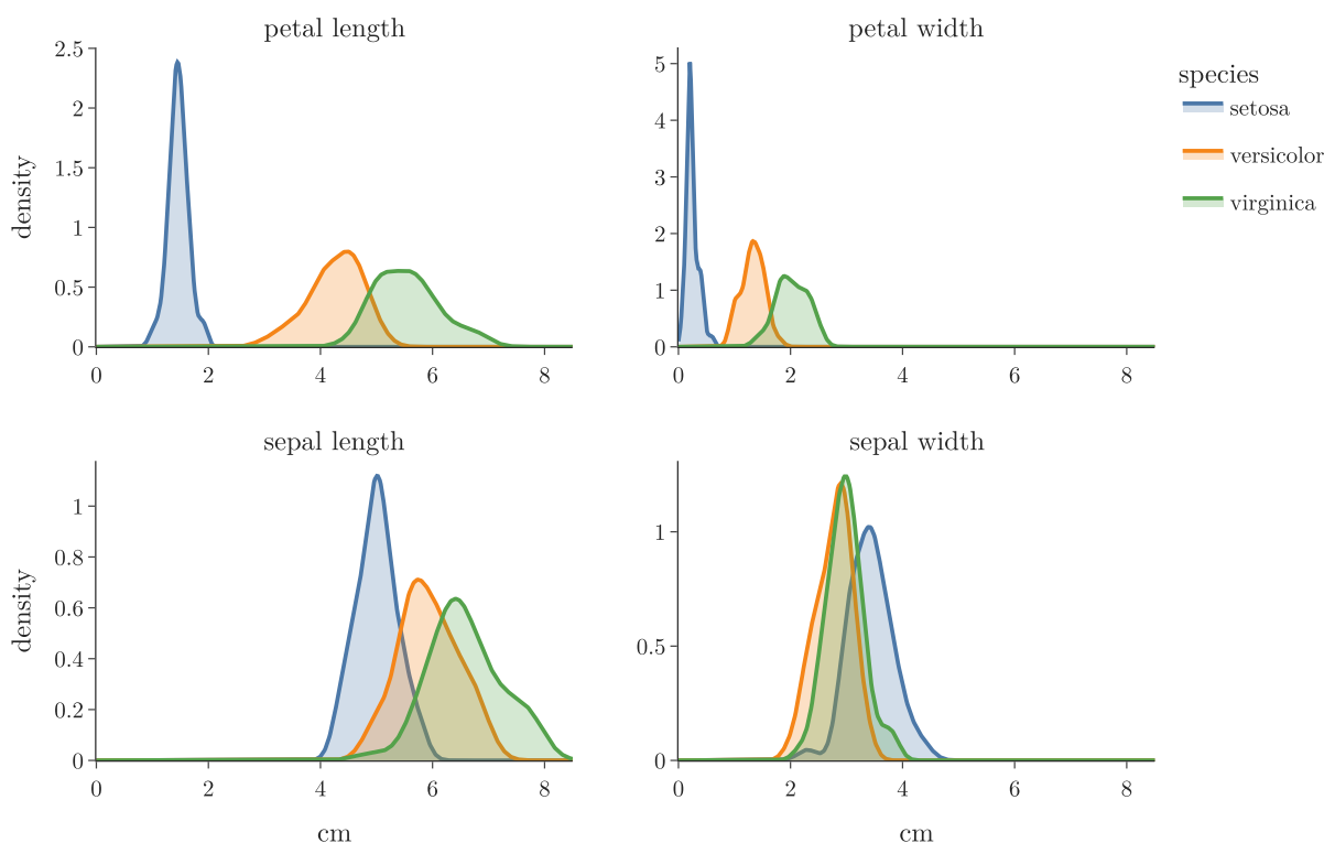
Figure 1: One density curve per iris species, for each of the four measurements
