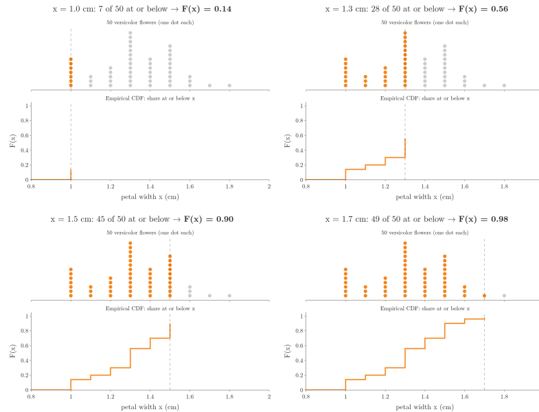
Figure 4: Building the empirical CDF of the 50 versicolor petal widths. At each cut-off x , the flowers at or below x turn orange and F(x) is their share; at 1.7 cm, 49 of 50 gives 0.98.
