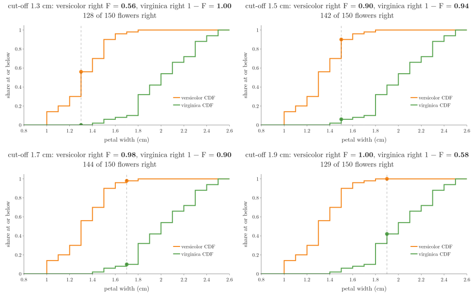
Figure 3: The cut-off slides from 1.3 to 1.9 cm across the versicolor (orange) and virginica (green) empirical CDFs. The dots give each class’s share at or below the cut-off; the title counts the flowers the rule gets right.
