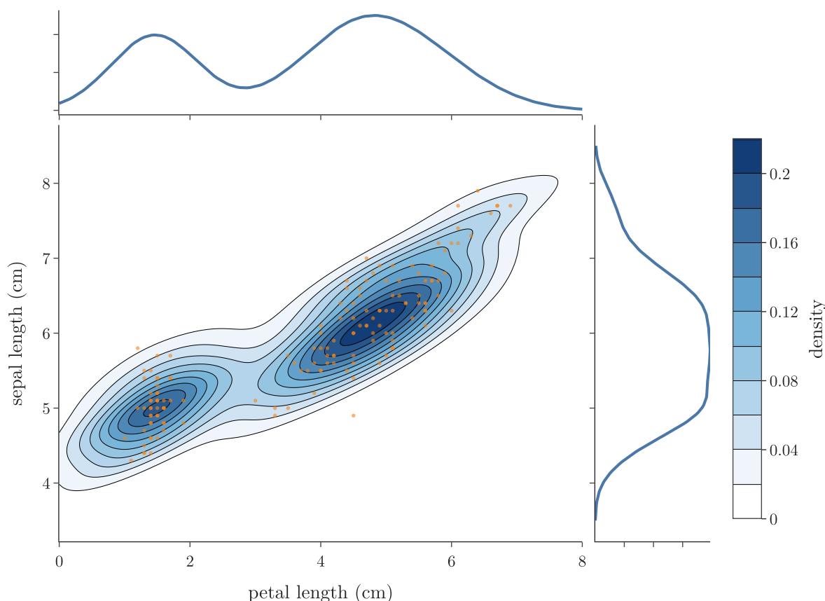
Figure 5: 2D density plot of petal length and sepal length, with each feature's 1D density on its edge
