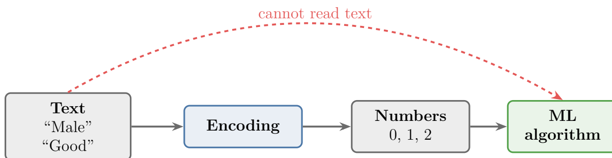
Figure 3: Encoding sits between text categories and the algorithm
