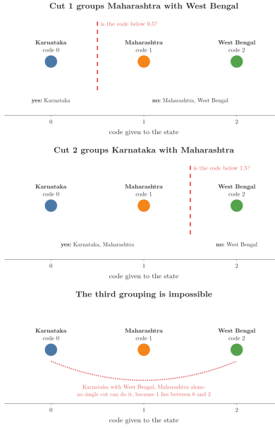
Figure 4: Three states numbered 0, 1, 2. One cut of the number line can form only two of the three possible groupings; which two depends only on the numbers we happened to choose. Idea after StatQuest, “One-Hot, Label, Target and K-Fold Target Encoding”.
