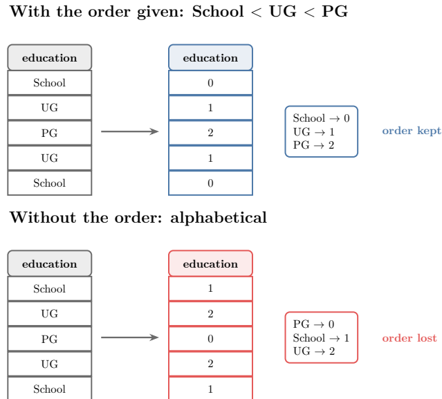
Figure 6: Ordinal encoding of the education column, with the order given (top) and without it (bottom)
