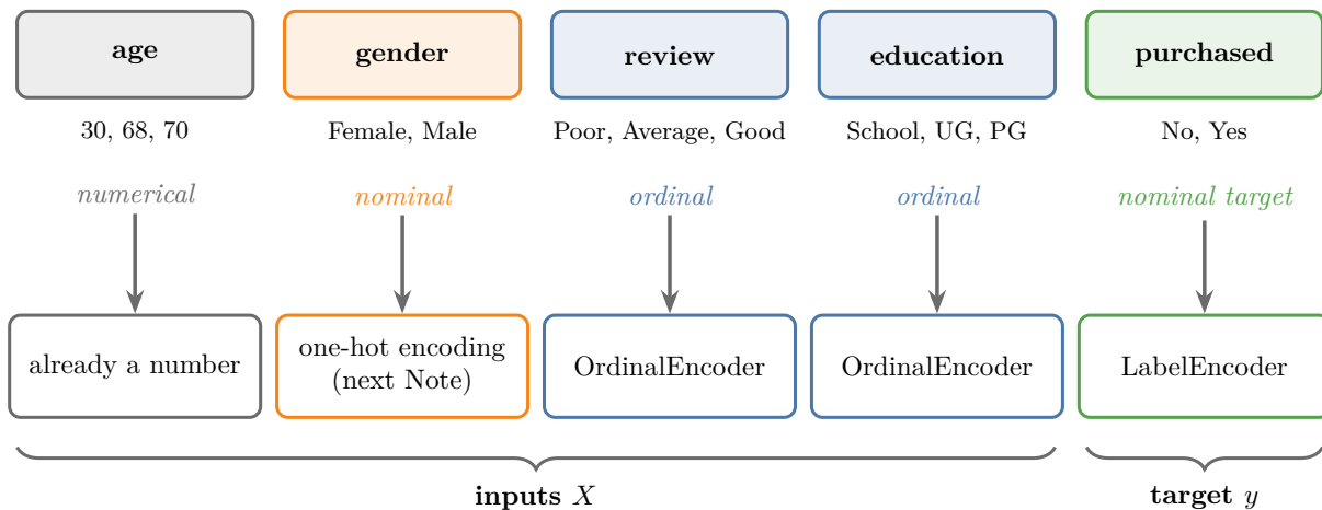
Figure 7: Each column of the customer data and the encoder it needs
