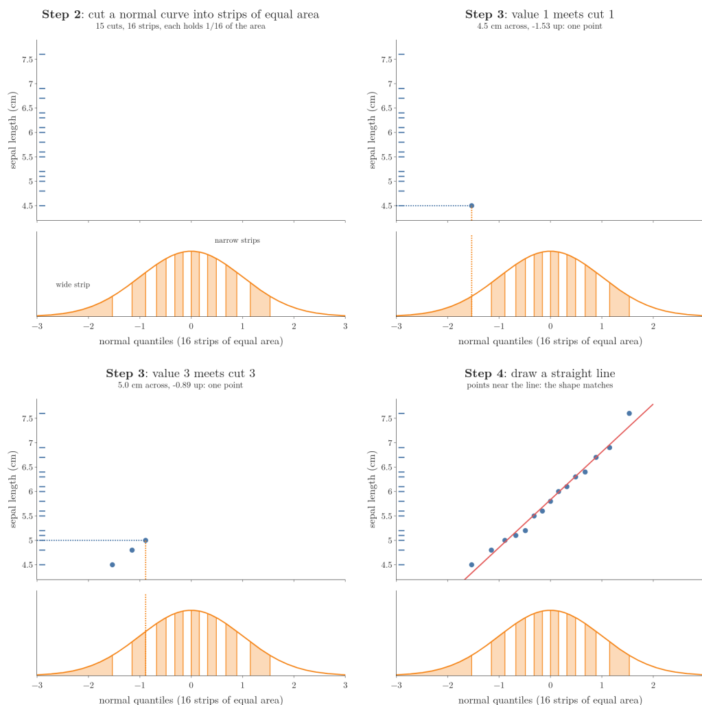
Figure 5: A Q-Q plot from 15 sepal lengths. A normal curve is cut into 16 strips of equal area; each cut (vertical dotted line) meets one sorted value (horizontal dotted line) at a point; a straight line is drawn through the 15 points. Idea after StatQuest, “Quantile-Quantile Plots (QQ plots), Clearly Explained!!!”.
