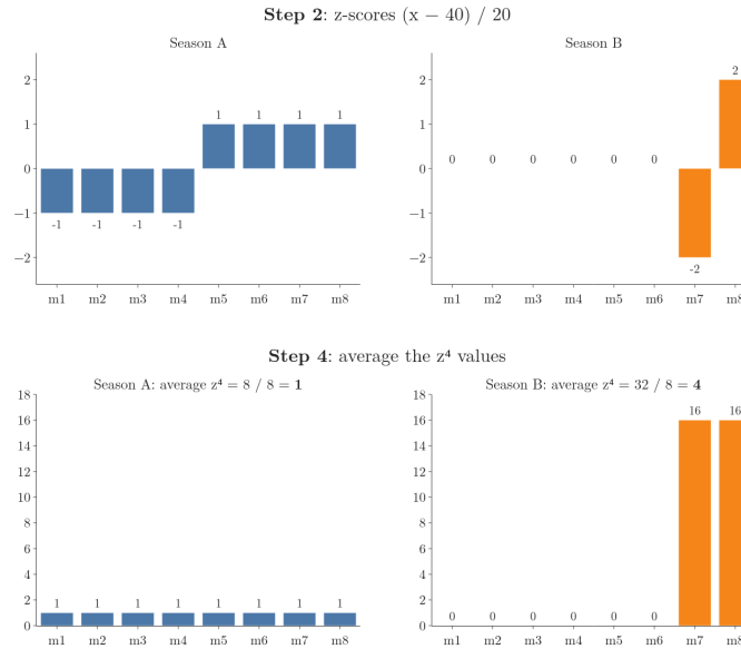
Figure 2: Kurtosis of the two 8-match seasons in steps: the scores, their z-scores, the fourth powers, and the average. Season A: eight 1s, kurtosis 1. Season B: two 16s and six 0s, kurtosis 4.
