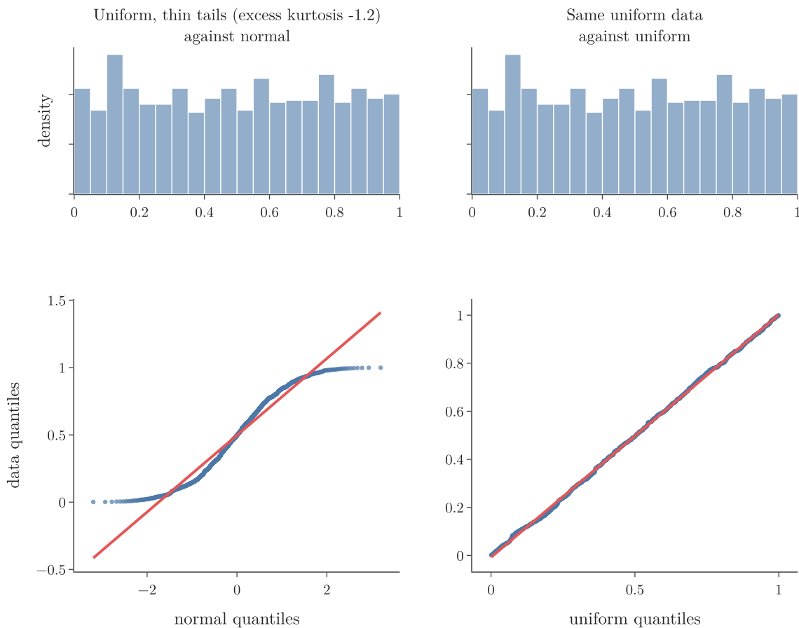
Figure 9: Top: histograms; bottom: Q-Q plots. Uniform data against the normal, then the same data against the uniform
