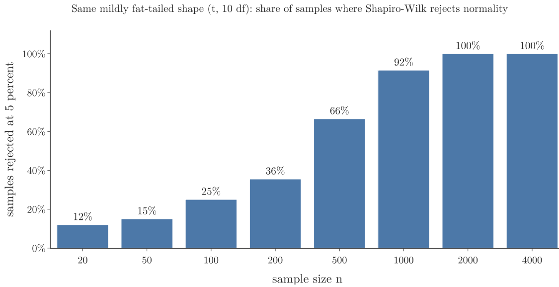
Figure 4: Share of 200 samples in which the Shapiro-Wilk test rejects normality at 5 percent, for samples of 20 to 4,000 values from the same mildly fat-tailed t distribution.
