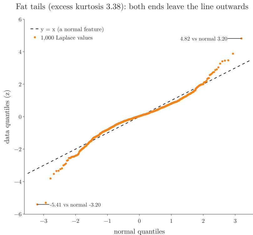
Figure 8: Q-Q plot of 1,000 standardized Laplace values against the normal. The middle follows the dashed line; both ends bend away from it, outwards.
