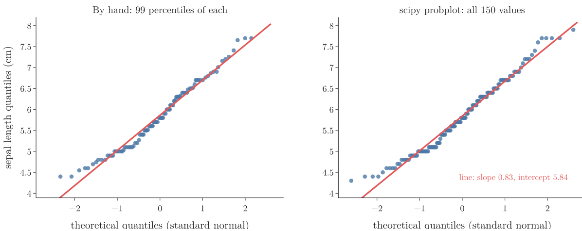
Figure 7: Q-Q plot of the iris sepal lengths against the normal distribution, by hand and with scipy
