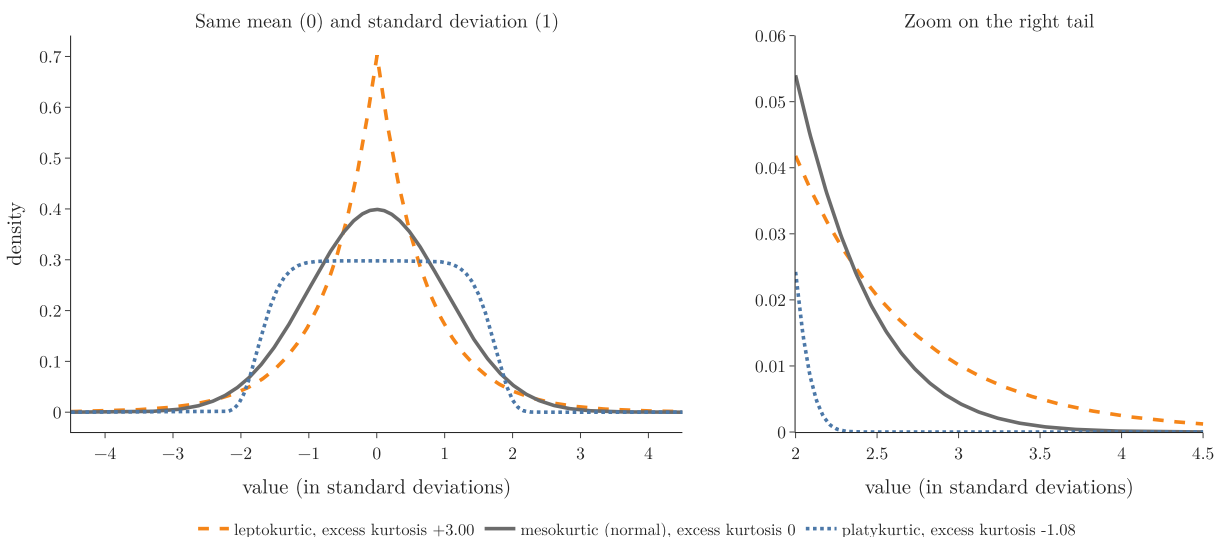
Figure 3: Three distributions with mean 0 and standard deviation 1 that differ only in their tails
