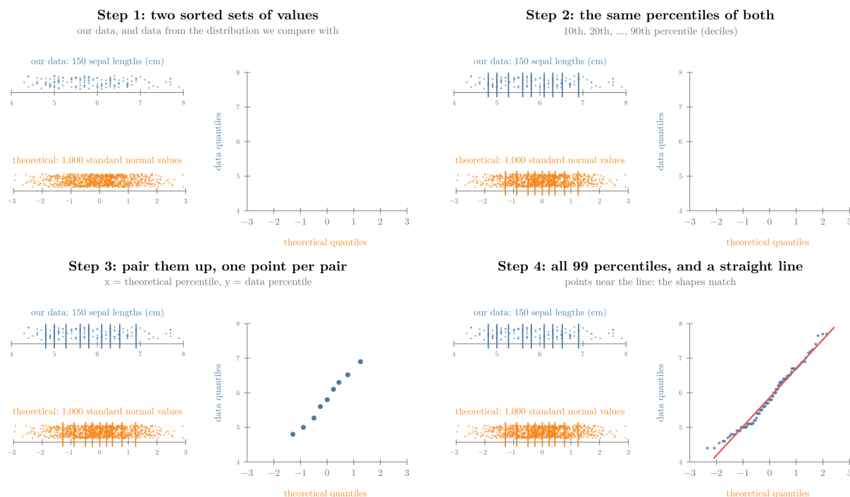
Figure 6: Building a Q-Q plot: sort both sets, take the same percentiles, plot them in pairs
