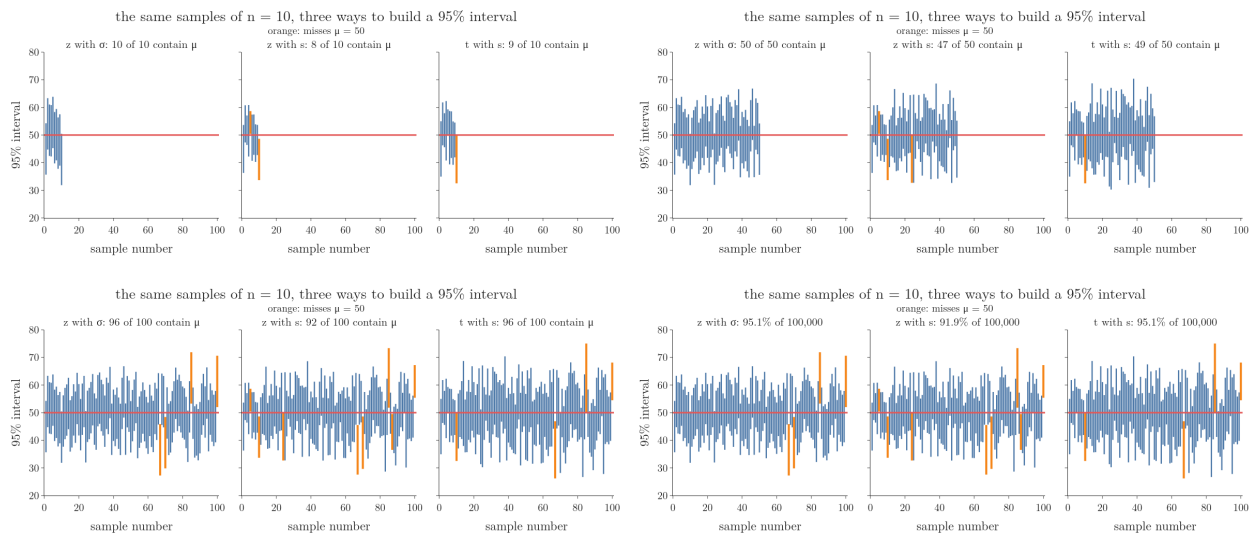
Figure 2: The same samples of n = 10 with three 95% intervals each: z with the true sigma, z with s, and t with s; misses in orange, running counts in the titles, coverage over 100,000 samples in the last frame (idea after Khan Academy, “Simulation showing value of t statistic”)
