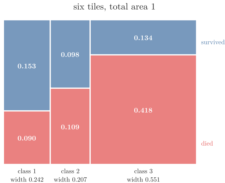
Figure 3: The joint distribution as a unit square: each class’s column is as wide as P(\text{class}) , and each tile’s area is a joint probability
