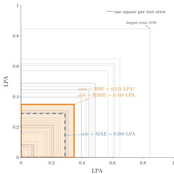
Figure 4: Each of the 40 test errors drawn as a square from the same corner (grey). Orange: the square whose area is the average area ( \text{MSE} = 0.121 \text{ LPA}^2 ); its side is \text{RMSE} = 0.348 \text{ LPA} . Dashed blue: the square whose side is the average side, \text{MAE} = 0.288 \text{ LPA} .
