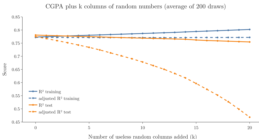
Figure 7: R^2 and adjusted R^2 as useless random features are added
