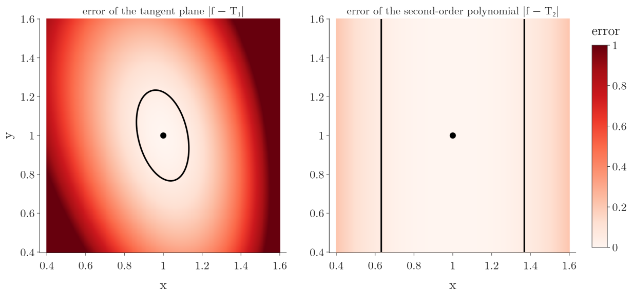
Figure 3: The size of the error near (1, 1) , on the same colour scale. Left: the tangent plane, |f - T_1| . Right: the second-order Taylor polynomial, |f - T_2| . The black line marks an error of 0.05; the region inside it is about nine times larger for T_2 .
