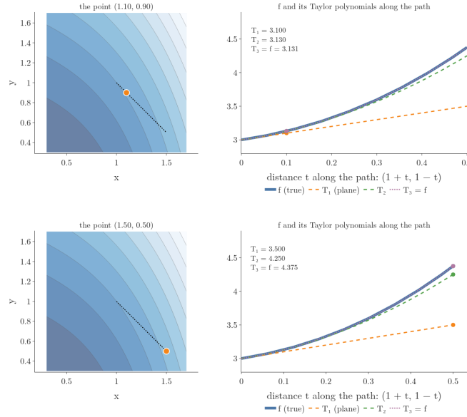
Figure 9: The Taylor polynomials of f(x, y) = x^3 + xy + y^2 around (1, 1) along the path to (1.5, 0.5) . Left: the moving point on the contour map. Right: f (thick blue) against T_1 , T_2 and T_3 ; T_3 equals f .
