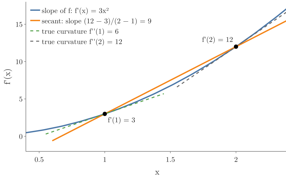
Figure 10: The secant idea for f = x^3 : the line through the slope readings at x = 1 and x = 2 has slope 9, a stand-in for the true curvatures 6 and 12
