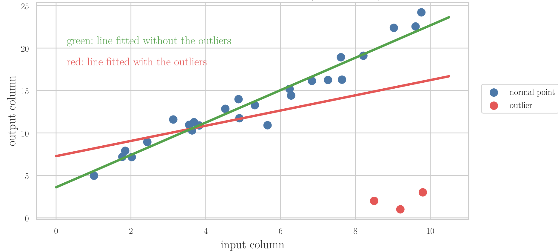
Three outliers pull the regression line (example data)
