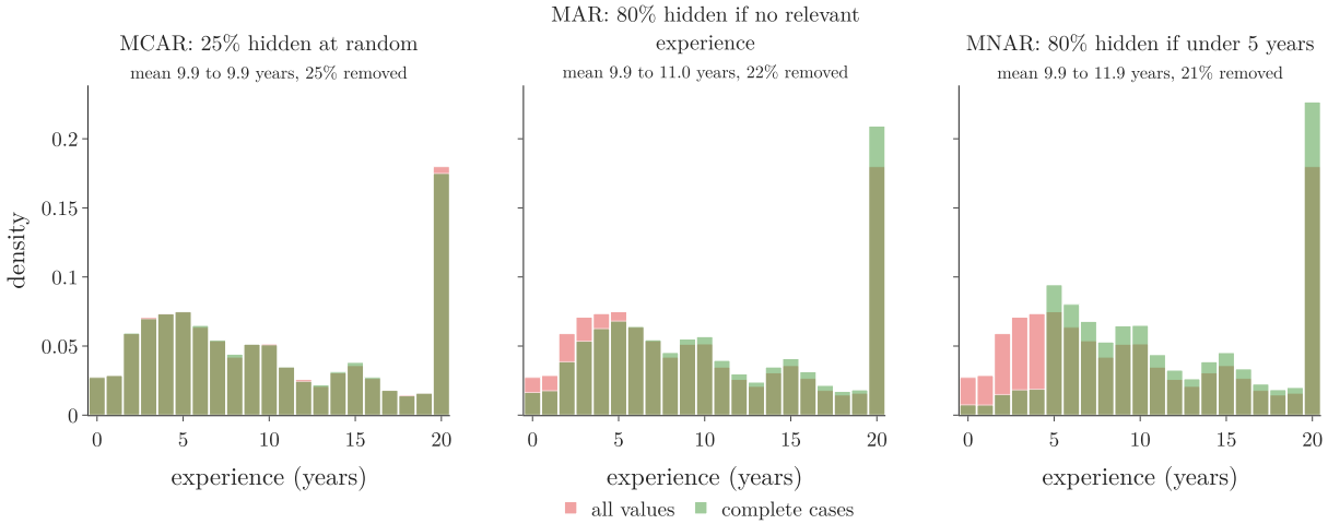
Figure 3: The experience column after hiding values in three ways: MCAR keeps the shape, while MAR and MNAR remove short experience and push the mean up
