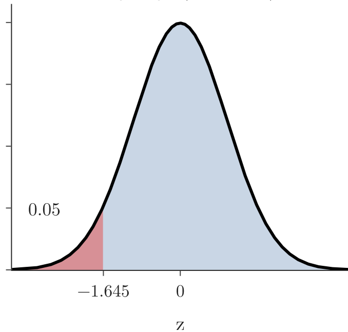
H_1: \mu < \mu_0 (left-tailed)
