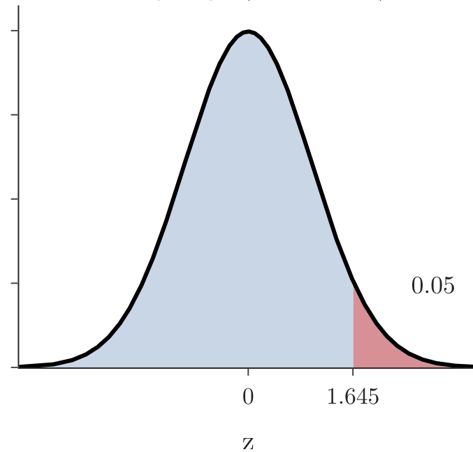
H_1: \mu > \mu_0 (right-tailed)
