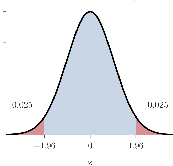
H_1: \mu \neq \mu_0 (two-tailed)
