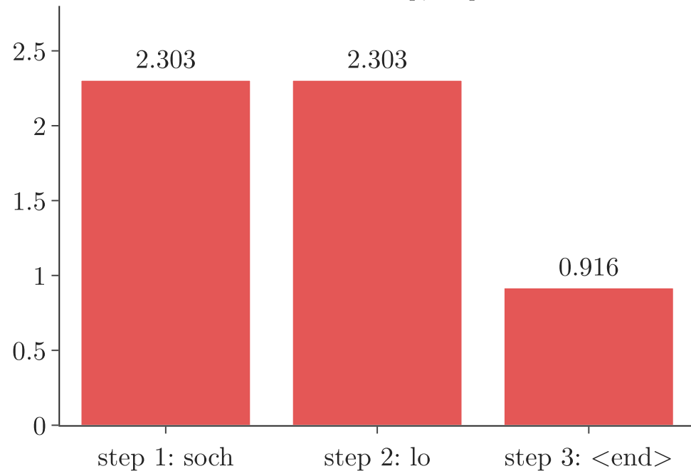
loss at the step, -\ln p
