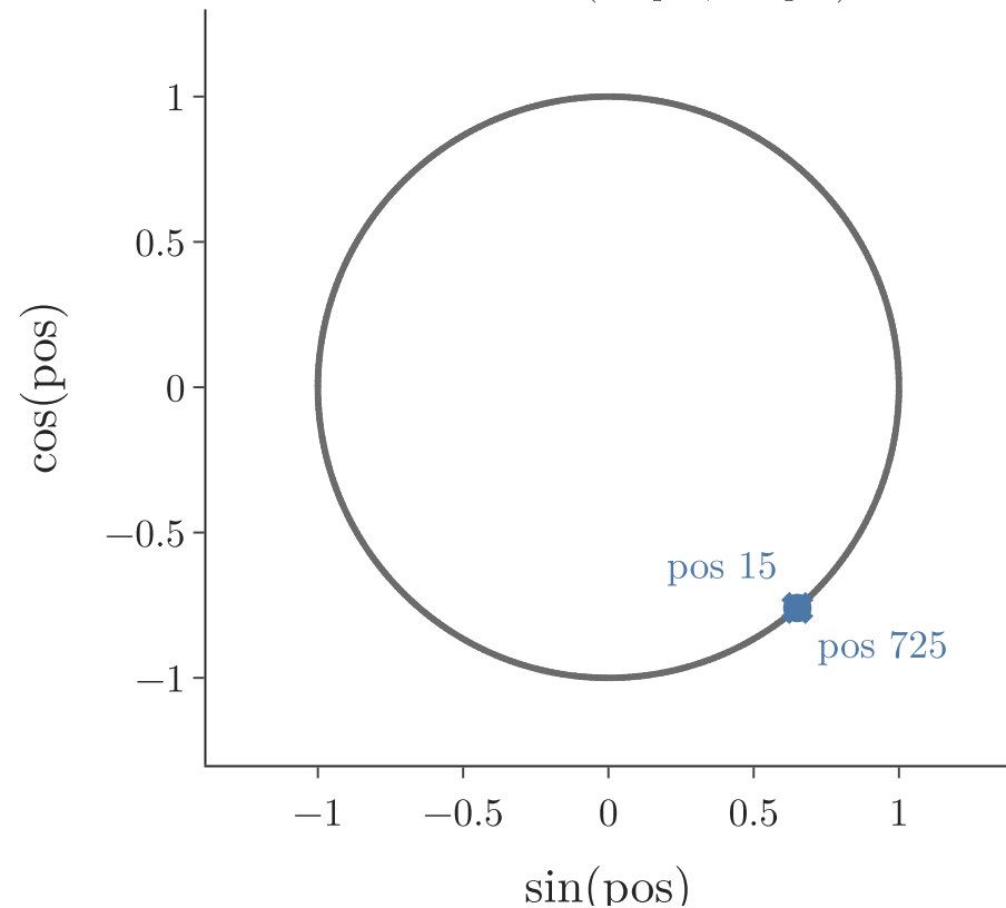
two numbers: (\sin \text{pos}, \cos \text{pos})
