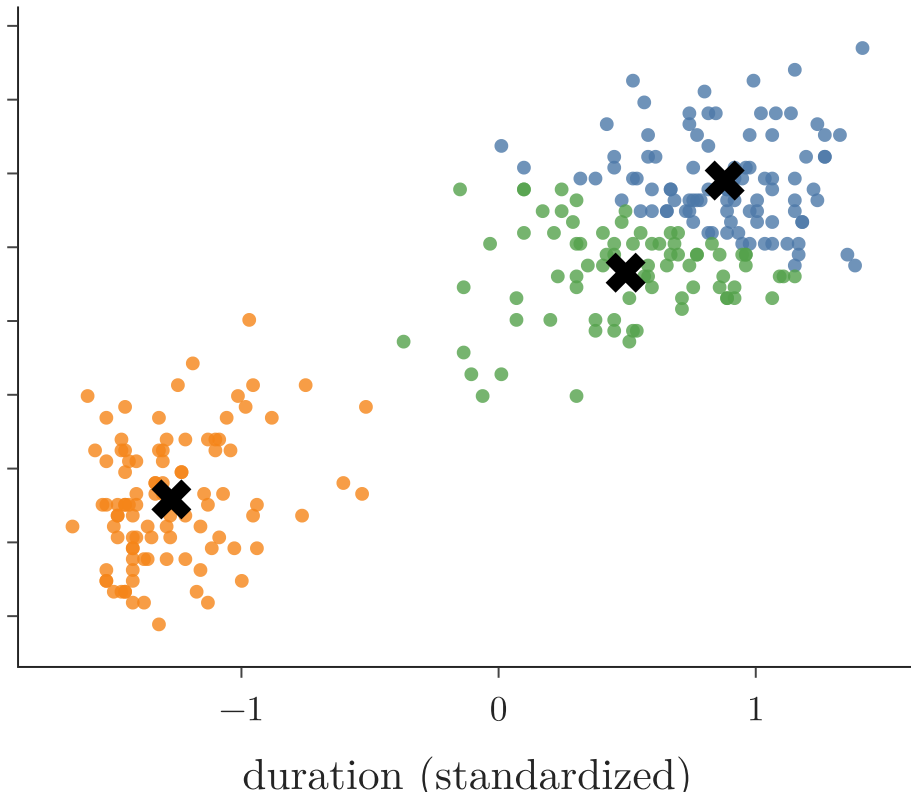
k = 3: WCSS 56; one group cut in two
