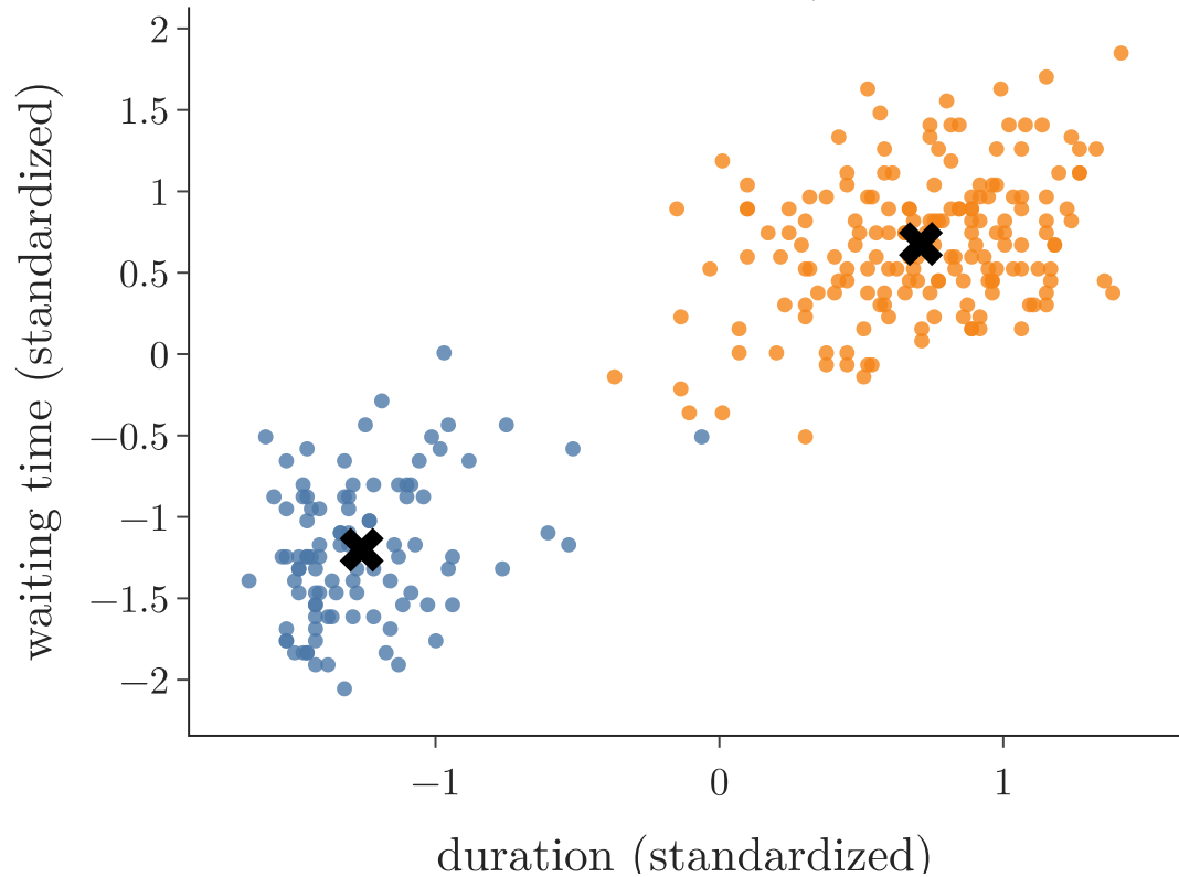
k = 2: WCSS 80; matches the short/long label for 99%
