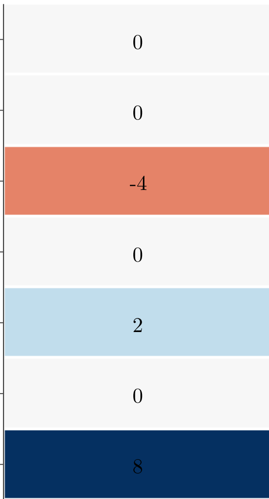
original 4 zeros of 7
