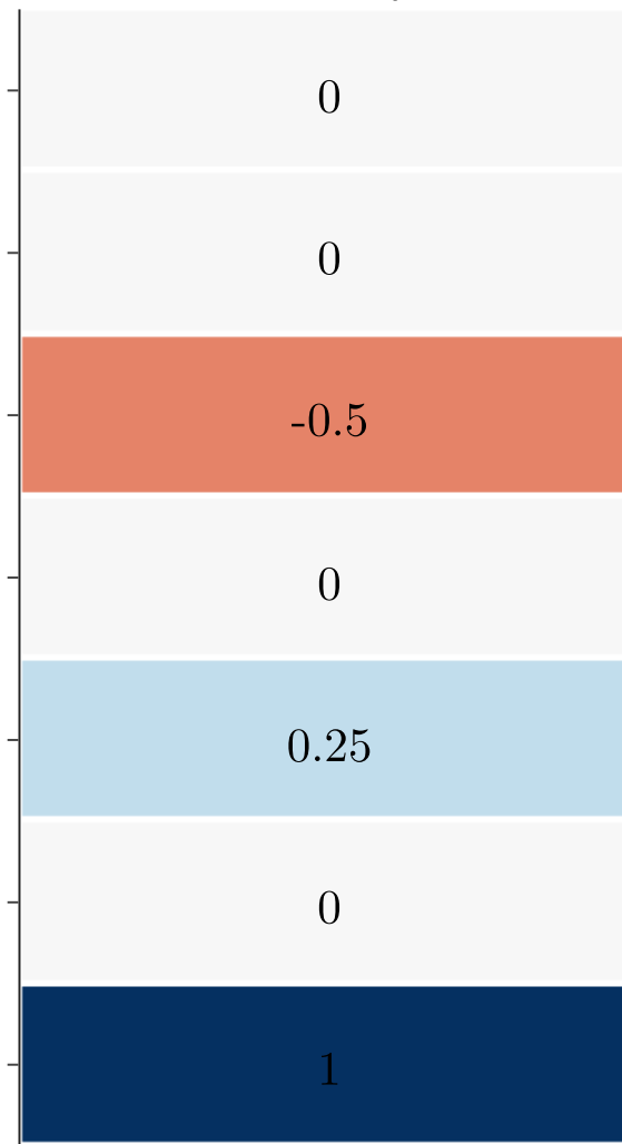
max-abs: divide by 8 zeros stay 0
