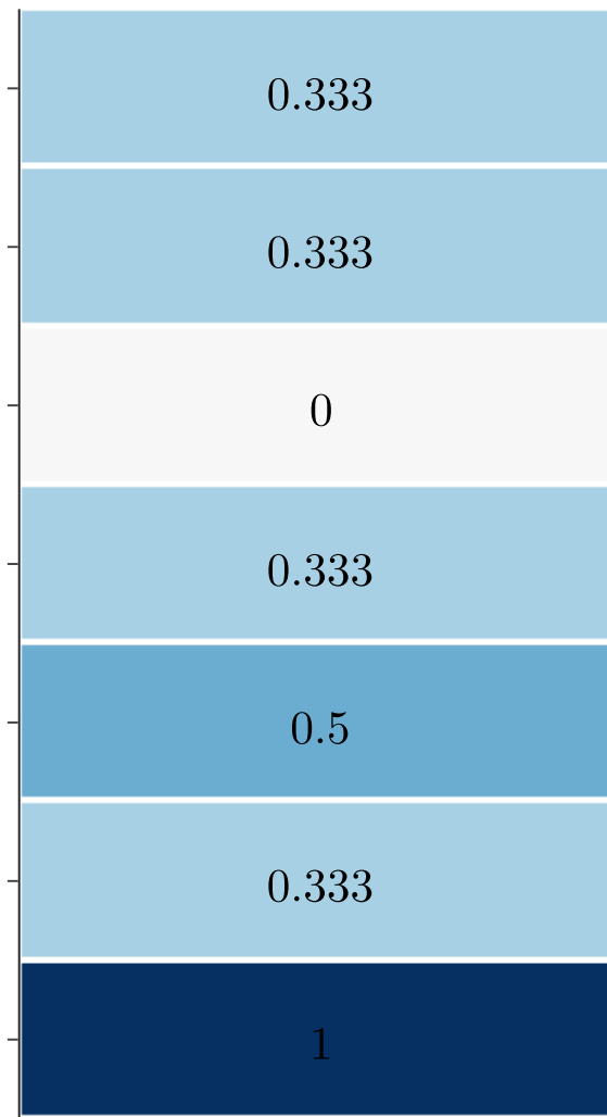
min-max zeros become 0.333
