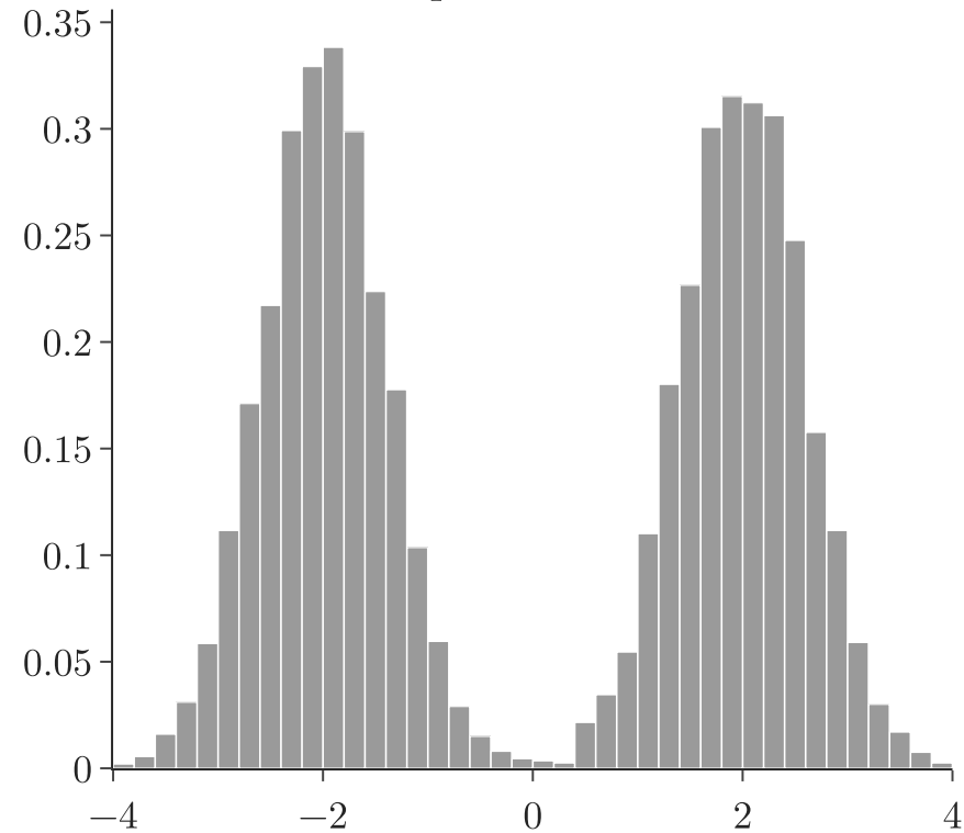
two humps: skewness +0.00
