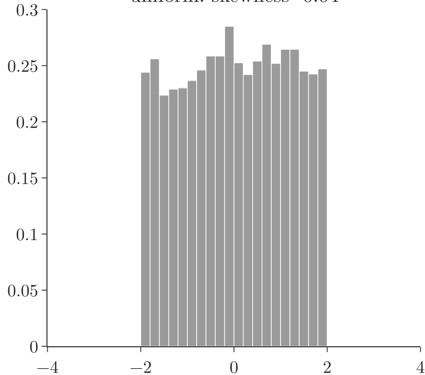
uniform: skewness -0.04
