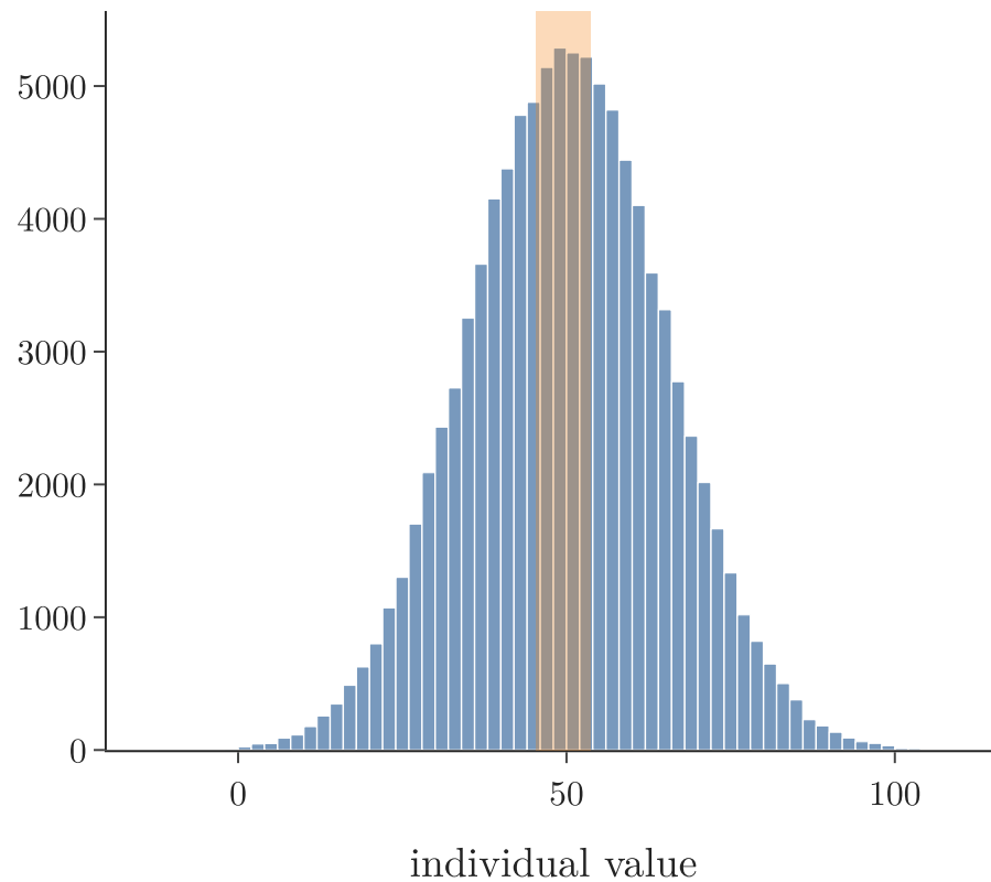
Misreading 3: individual values 21.7% inside this interval
