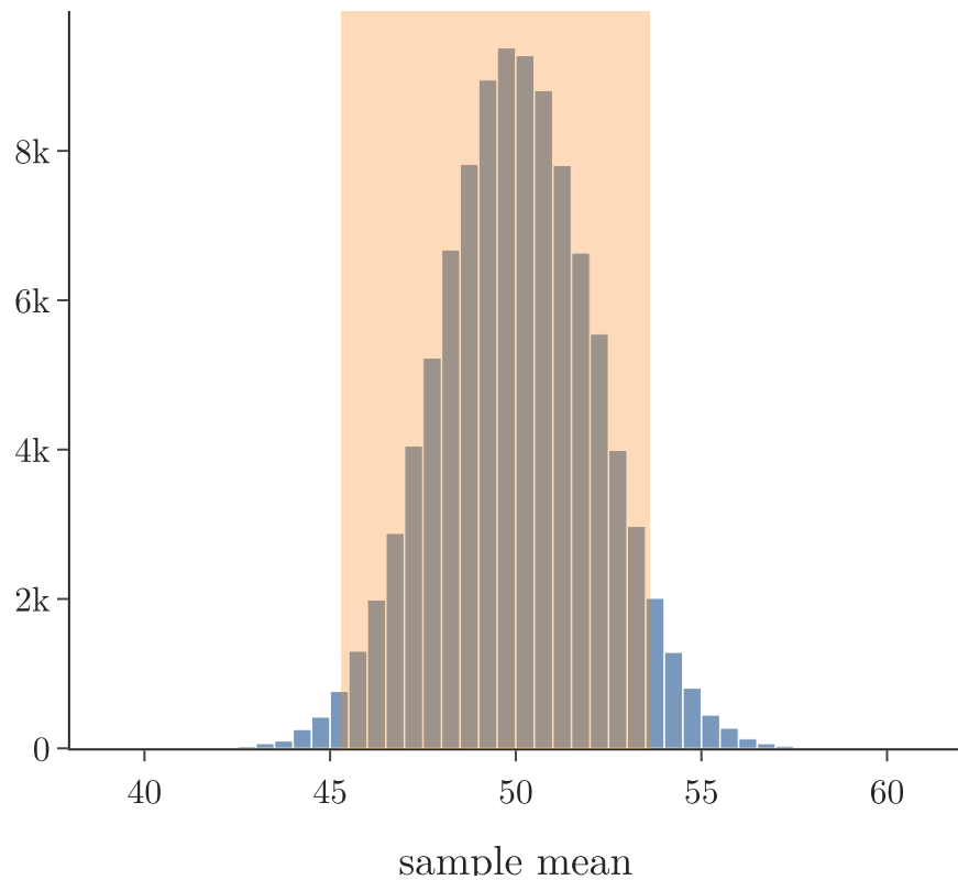
Misreading 2: new sample means 94.2% inside this interval
