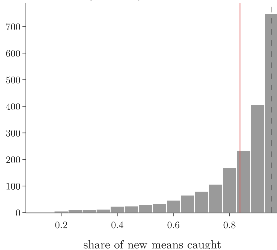
Many first samples: share of new means caught averages 0.837 , not 0.95
