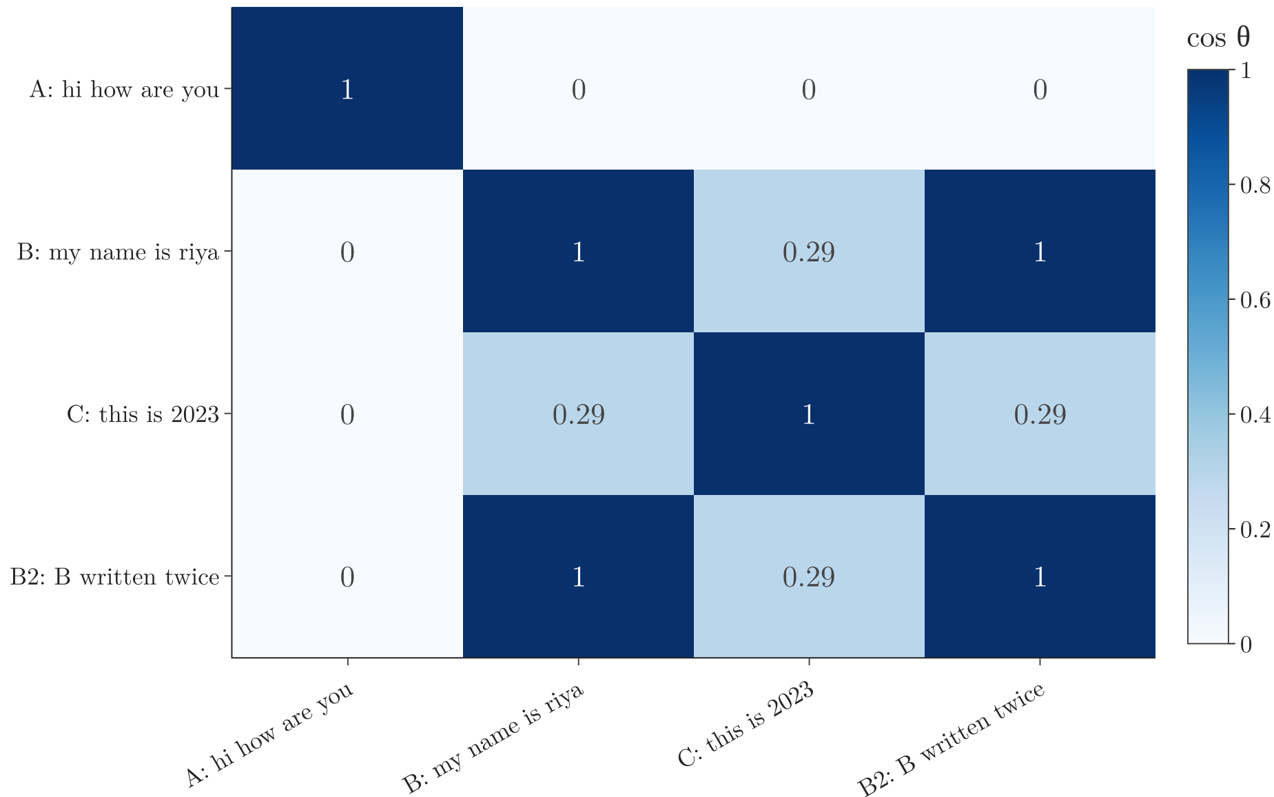
Cosine similarity of word-count vectors
