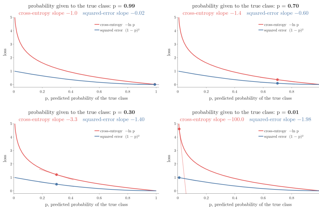
Figure 9: The probability p given to the true class slides from 0.99 to 0.01. Red: cross-entropy and its tangent. Blue: the squared error and its tangent. The title prints both slopes. Idea after StatQuest, “Neural Networks Part 6: Cross Entropy”
