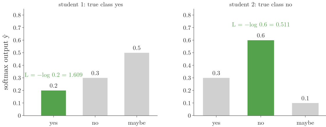
Figure 11: Softmax outputs of the two students; only the true class (green) enters the loss
