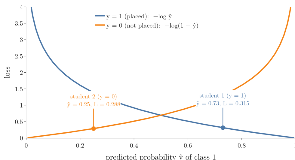
Figure 8: The loss for each label as the predicted probability changes, with the two students marked
