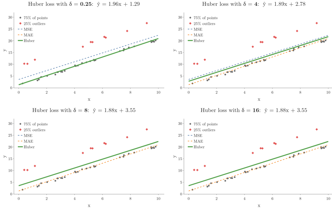
Figure 7: The Huber line (green) refitted on the 40 points of Figure 6 as \delta grows from 0.25 to 16, with the MSE and MAE lines dashed
