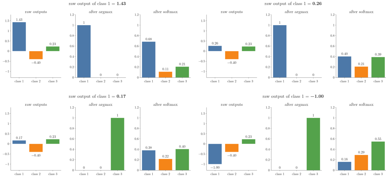
Figure 10: Three raw outputs (left), after argmax (middle) and after softmax (right), while the raw output of class 1 slides from 1.43 down to -1 . Idea after StatQuest, “Neural Networks Part 5: ArgMax and SoftMax”
