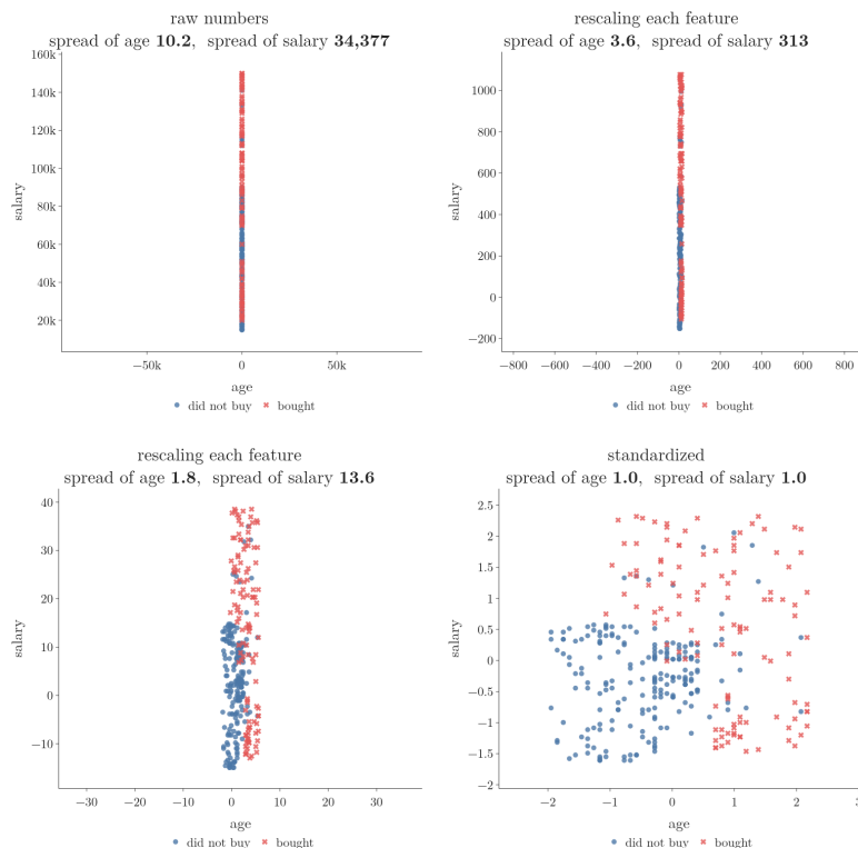
Figure 6: The 320 training users while each feature has its mean removed and is divided by its standard deviation. One unit has the same length on both axes. The title gives the standard deviation (spread) of each feature
