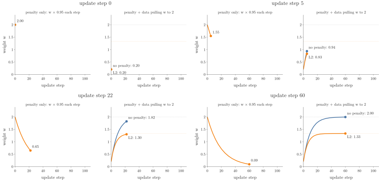
Figure 4: Weight decay on one weight, \eta = 0.1 , \lambda = 0.5 . Left: the penalty alone multiplies the weight by 0.95 at every step. Right: with a data loss that pulls the weight to 2, the weight without a penalty (blue) reaches 2, and the weight with L2 (orange) settles lower, at 1.33
