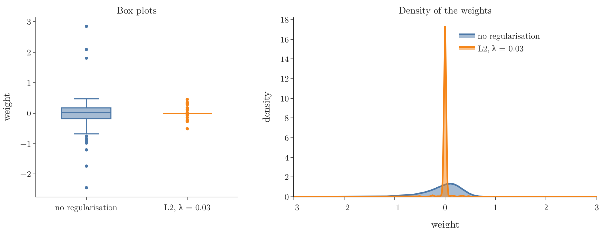
Figure 6: The 256 first-layer weights without regularisation and with L2. Left: box plots. Right: density curves.
