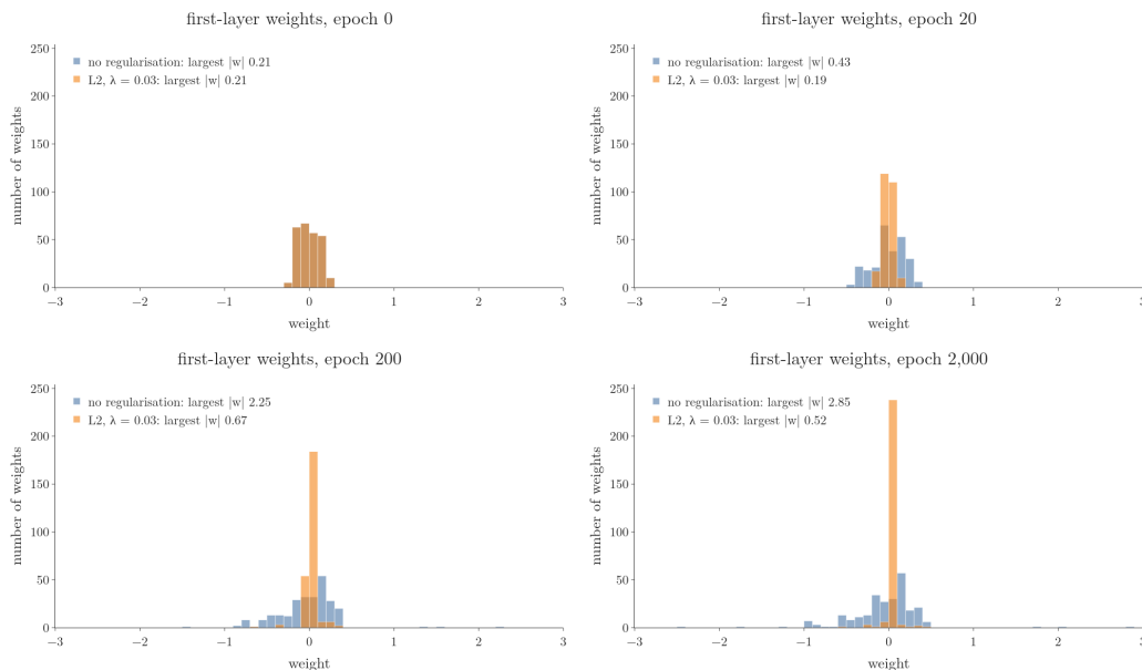
Figure 7: The 256 first-layer weights during training, same start: without regularisation (blue) they spread out, up to 2.85 in size; with L2, \lambda = 0.03 (orange), they stay in a spike around 0
