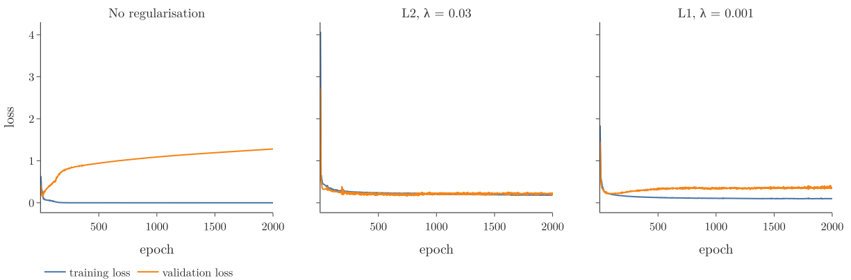
Figure 5: Training and validation loss over 2,000 epochs: without regularisation, with L2 and with L1.
