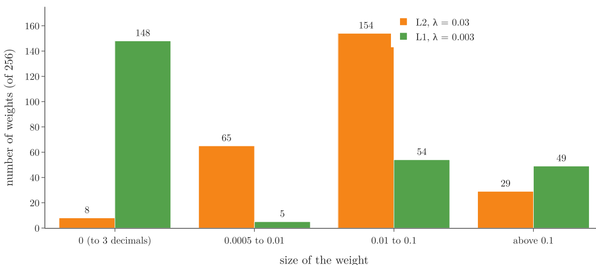
Figure 8: The 256 first-layer weights after 2,000 epochs of plain gradient descent, grouped by size: L2 (orange) and L1 (green), first random start.
